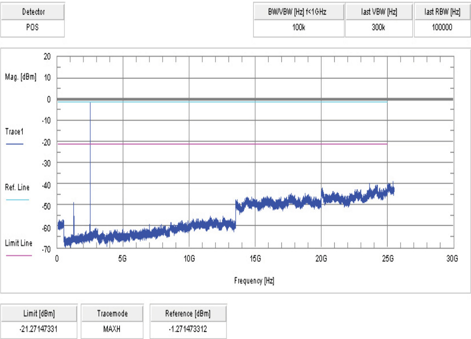
Plot 3: highest channel
