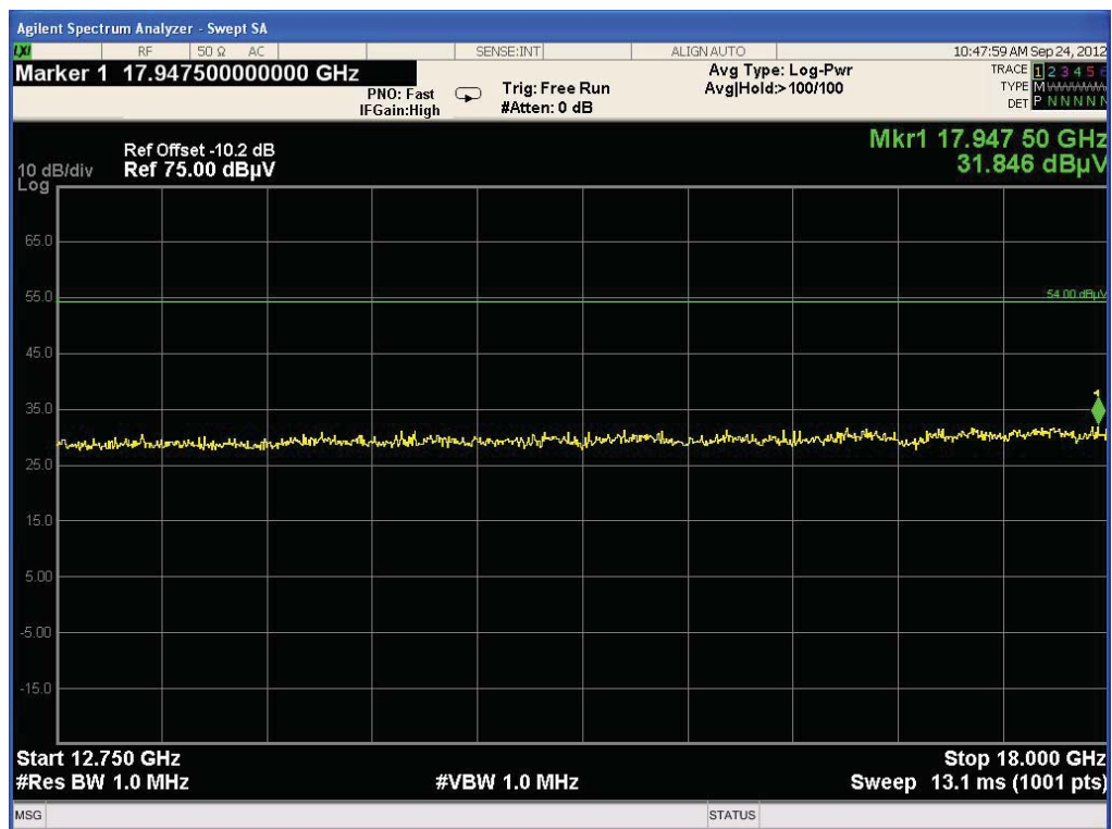
Plot 3: 12.75 GHz to 18 GHz, lowest channel, vertical & horizontal polarization
