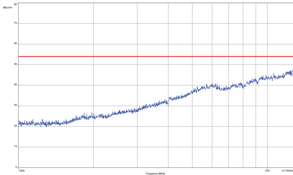
Plot 2: 1 GHz to 12.75 GHz, RX / idle – mode, vertical & horizontal polarization
