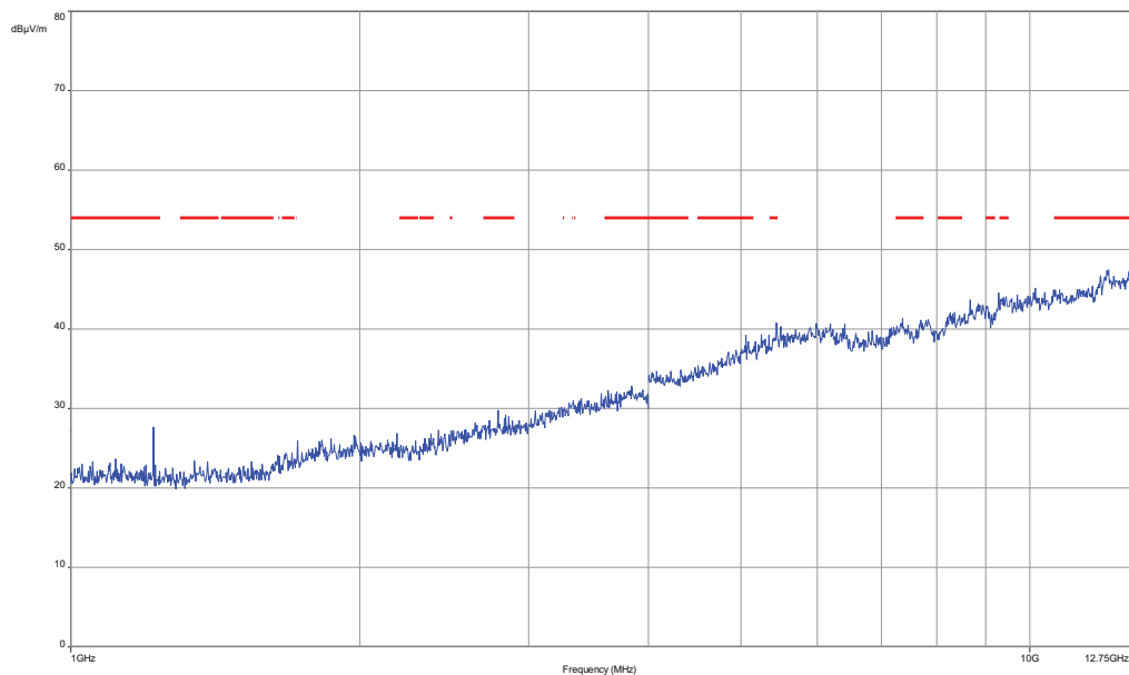
Plot 6: 1 GHz to 12.75 GHz, mid channel, vertical & horizontal polarization
