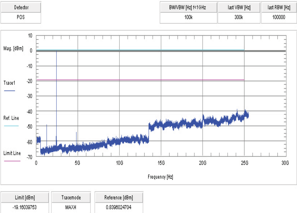
Plot 1: lowest channel
