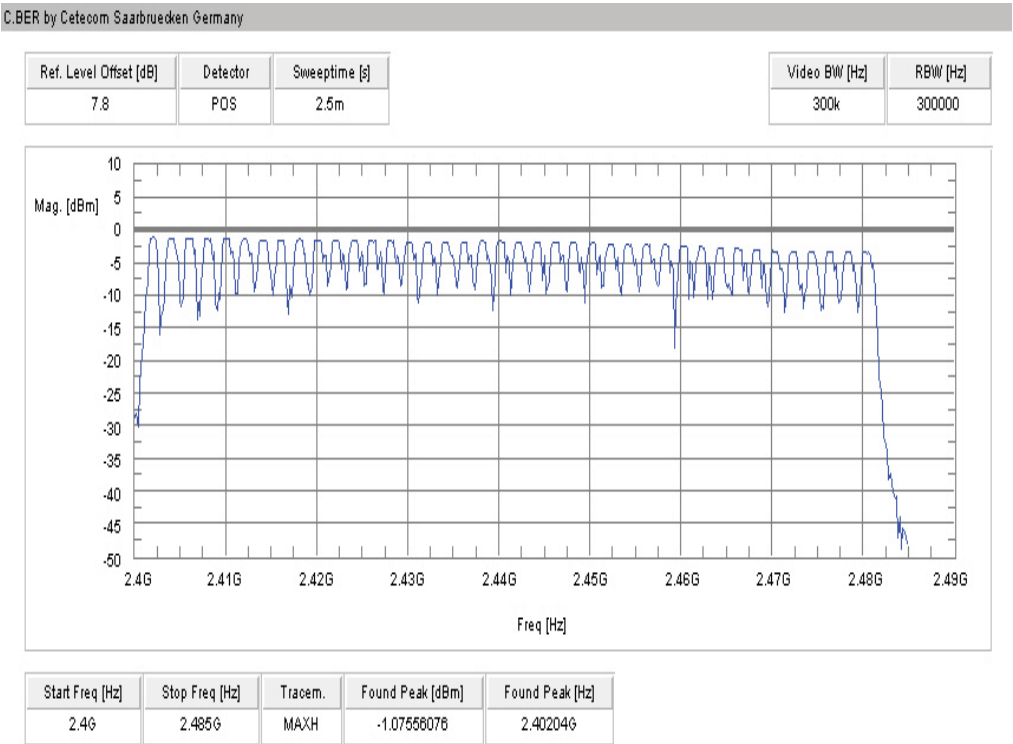
Plot 1: Number of hopping channels
