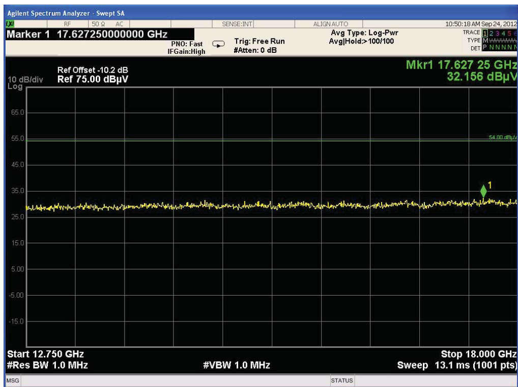
Plot 11: 12.75 GHz to 18 GHz, highest channel, vertical & horizontal polarization
