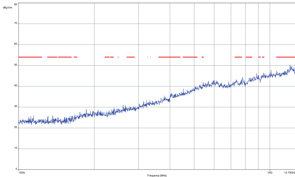
Plot 10: 1 GHz to 12.75 GHz, highest channel, vertical & horizontal polarization
