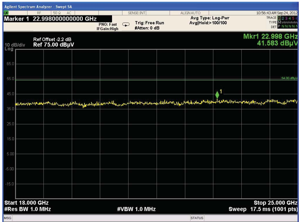
Plot 4: 18 GHz to 25 GHz, RX / idle – mode, vertical & horizontal polarization
