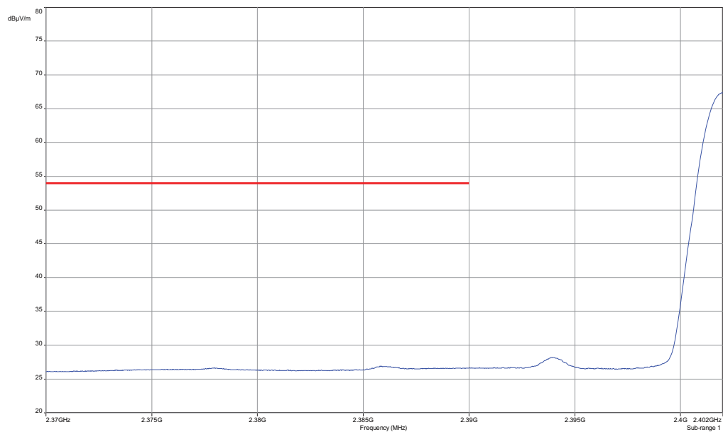
Plot 1: Lower restricted band
