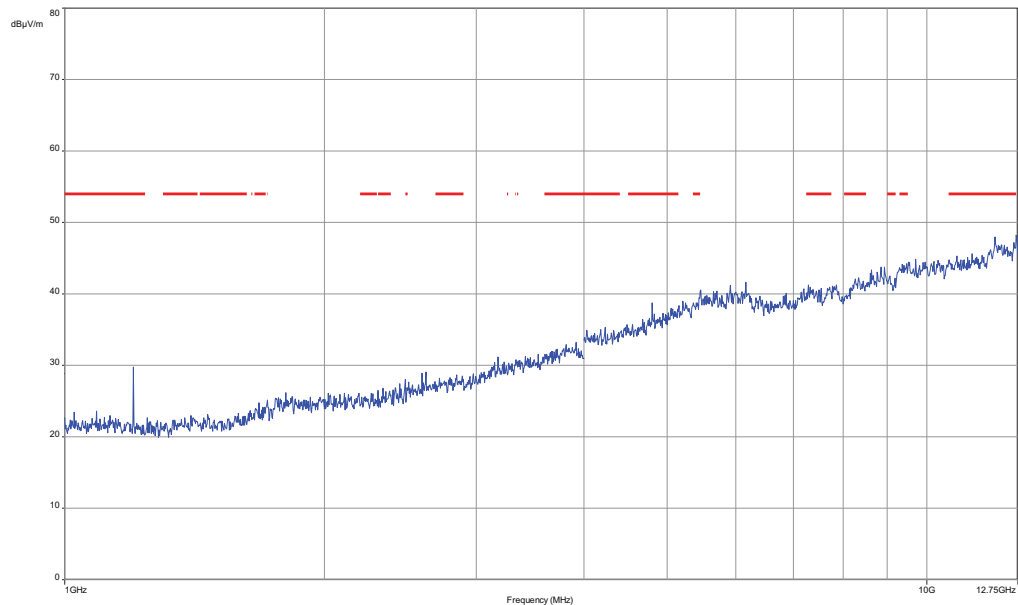
Plot 2: 1 GHz to 12.75 GHz, lowest channel, vertical & horizontal polarization
