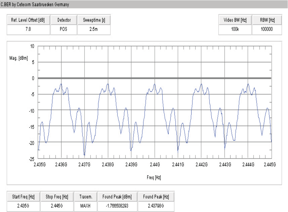
Plot 1: Carrier Frequency Separation
