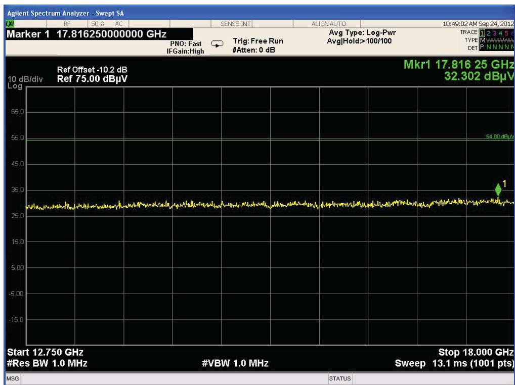
Plot 7: 12.75 GHz to 18 GHz, mid channel, vertical & horizontal polarization
