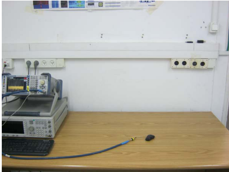
Figure 4. Conducted Emission Test
