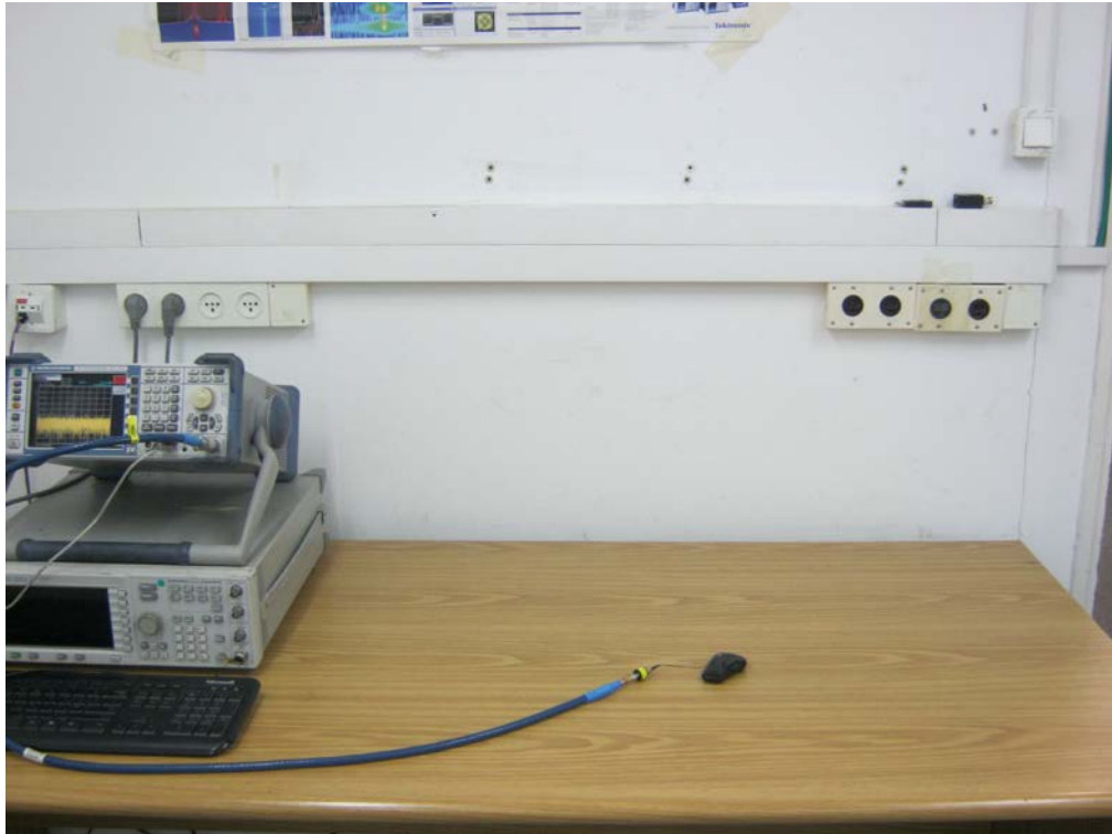
Figure 4. Conducted Emission Test
