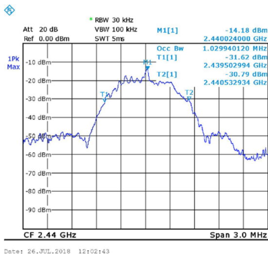
Figure 10. BLE, Mid
