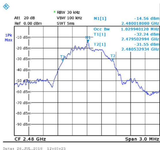
Figure 11. BLE, High
