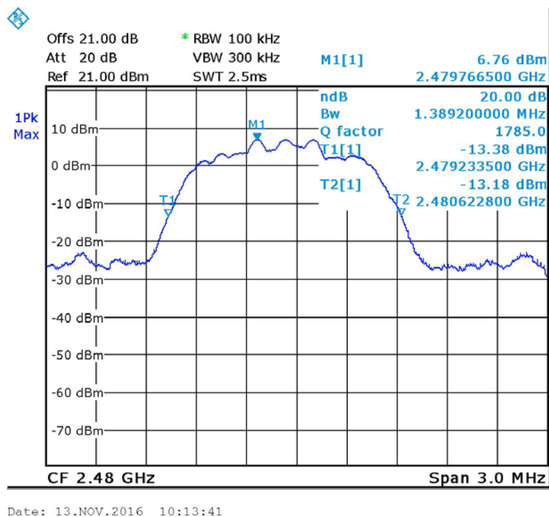
Figure 21. 2480- High EDR Modulation
