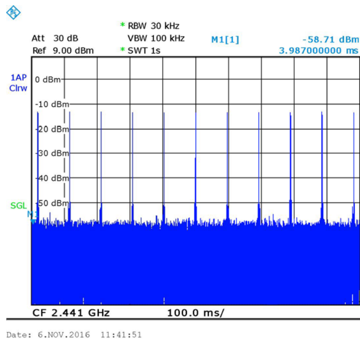
Figure 50 — Number of Bursts in 1 sec=11 standard modulation
