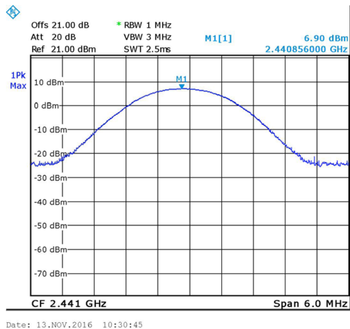
Figure 28 — 2441 - Mid EDR Modulation
