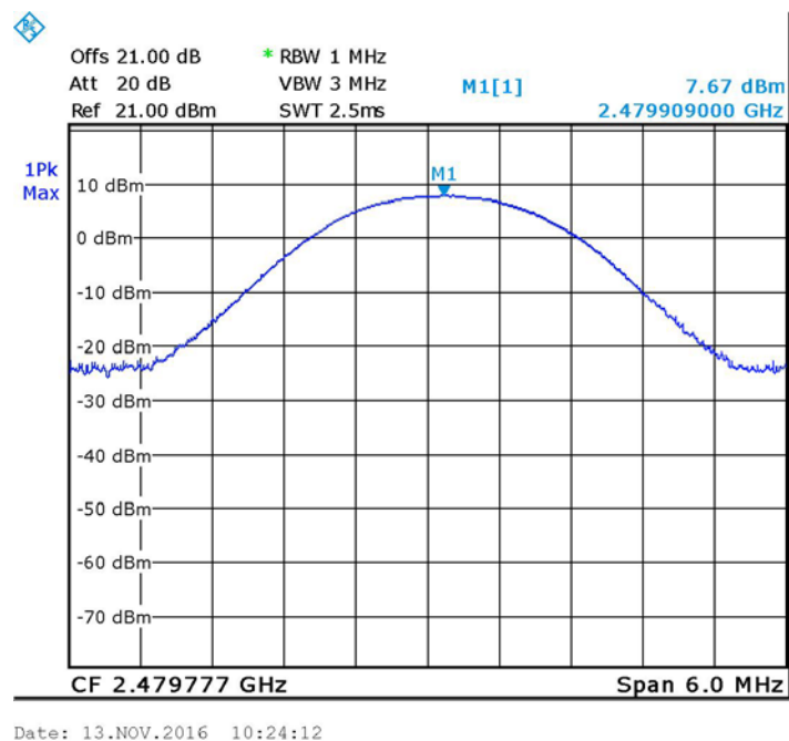
Figure 29 — 2480MHz - High EDR Modulation
