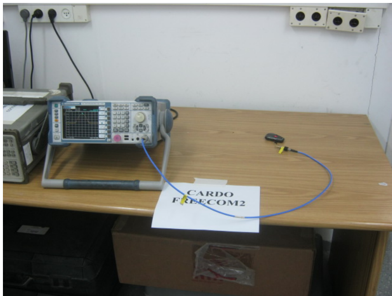
Conducted Emission From Antenna Ports Test Set-Up
