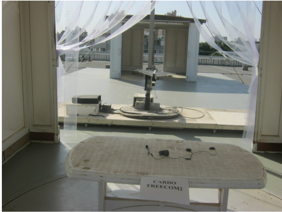
Radiated Emission Test- 200MHz-1000MHz
