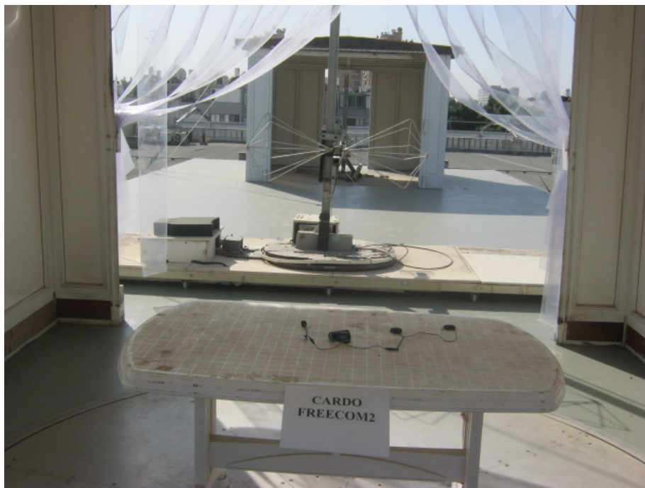
Radiated Emission Test- 30MHz-200MHz
