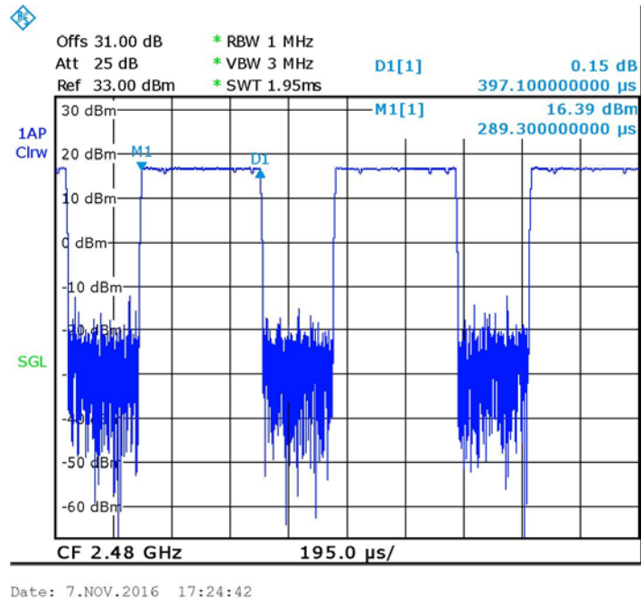
Figure 48. Burst Duration
