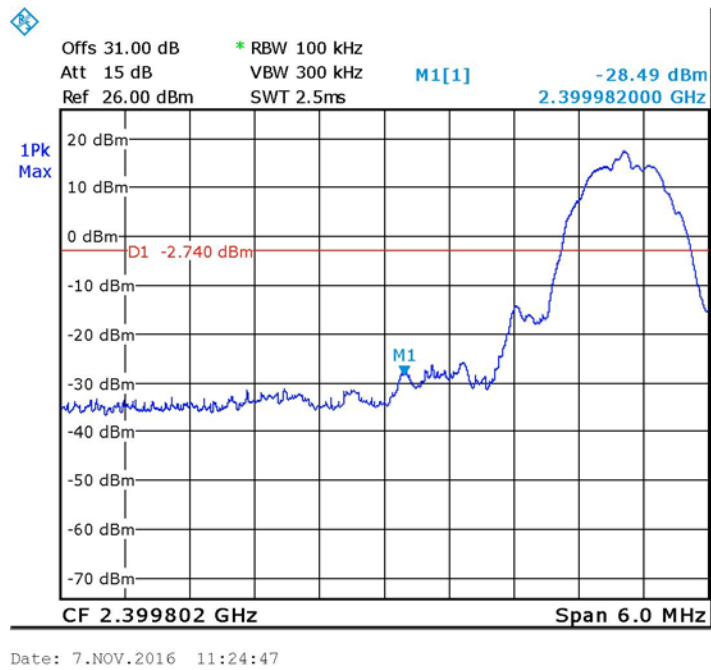
Figure 32 —Lower Band Edge
