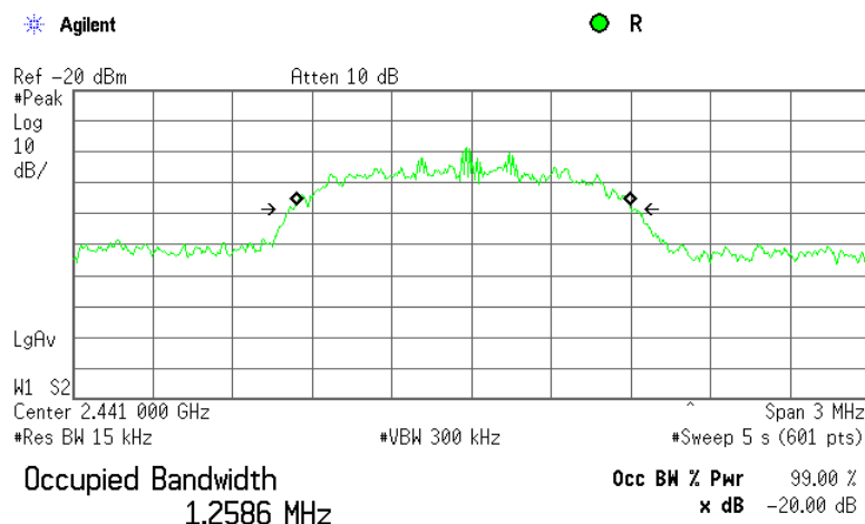
Plot 7.1.5 The occupied bandwidth test result at mid frequency, DQPSK modulation
