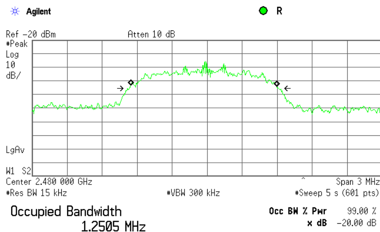
Plot 7.1.6 The occupied bandwidth test result at high frequency, DQPSK modulation
