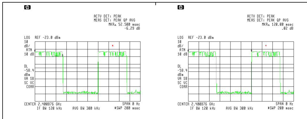
Figure 32. Duty Cycle
