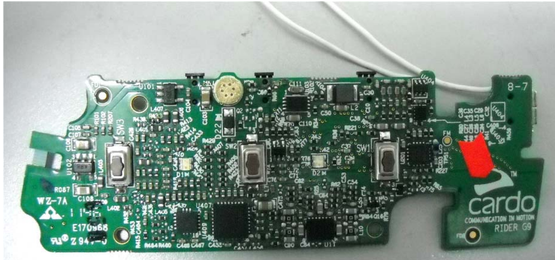
Photograph No.6 Bluetooth headset PCB second side view
