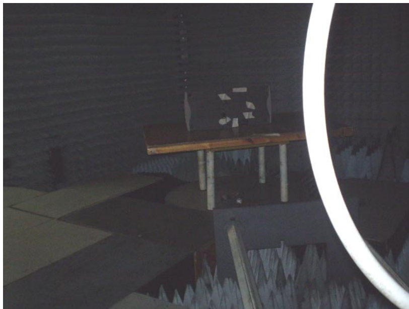
Photograph No.2 Spurious emissions field strength measurement setup in the anechoic chamber below 30 MHz
