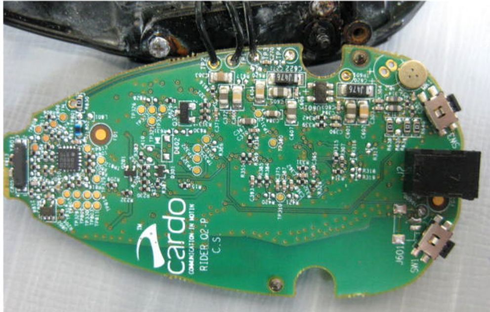
Photograph No.3 Bluetooth headset PCB second side view
