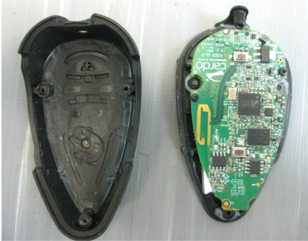
Photograph No.1 Bluetooth headset internal view
