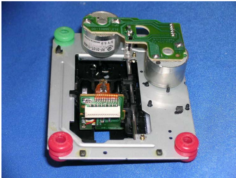
CD loader rear side (View 3)
