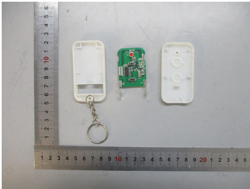
EUT(BH18D) – PCB Top View
