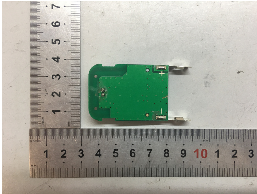
EUT(BH18D) – PCB Bottom View
