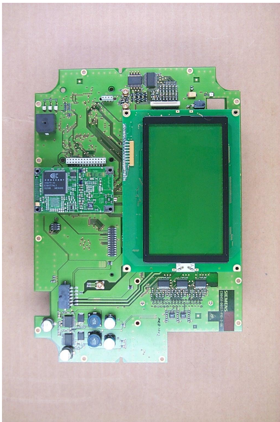
20608eut14.jpg: X-Pack DS, main board, front view (with display and gps-receiver)
