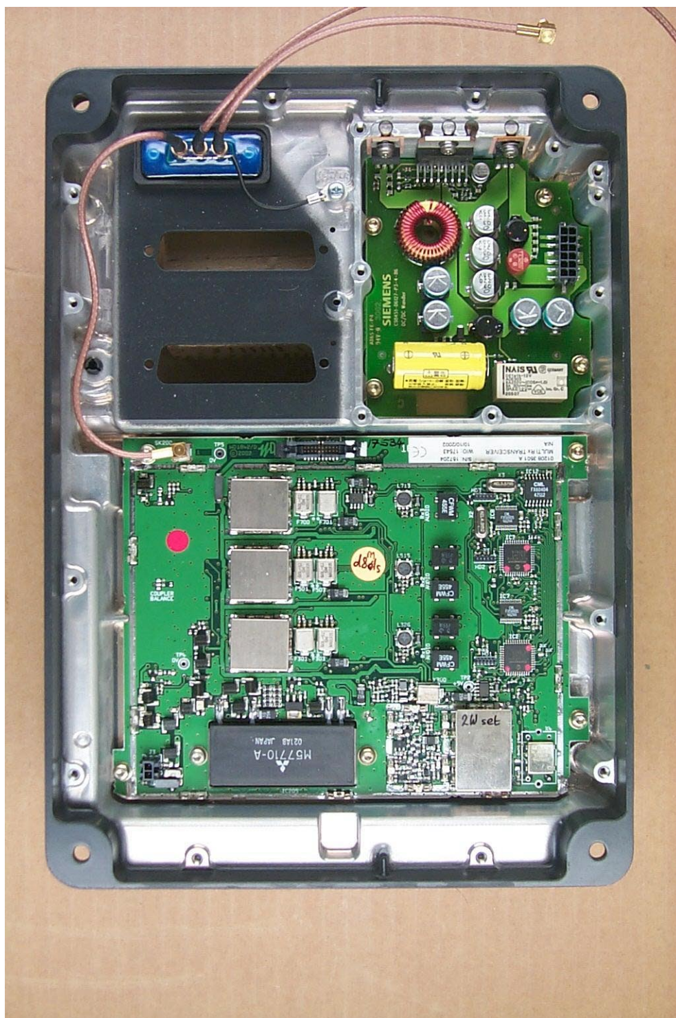
20608eut6.jpg: X-Pack DS, inside view (power supply and rf-part)
