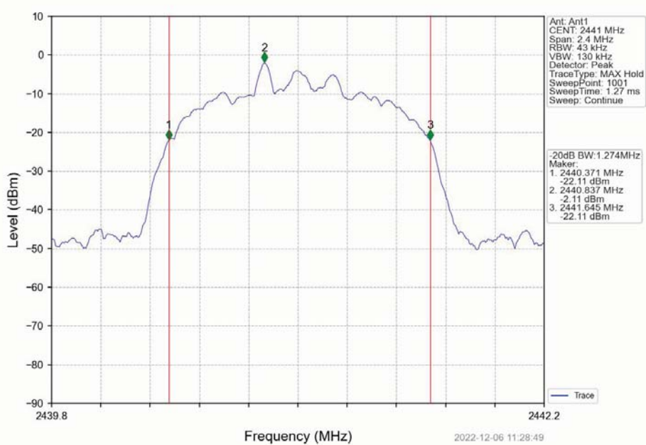
8DPSK_3DH5_MCH_2441MHz_Ant1_NTNV
