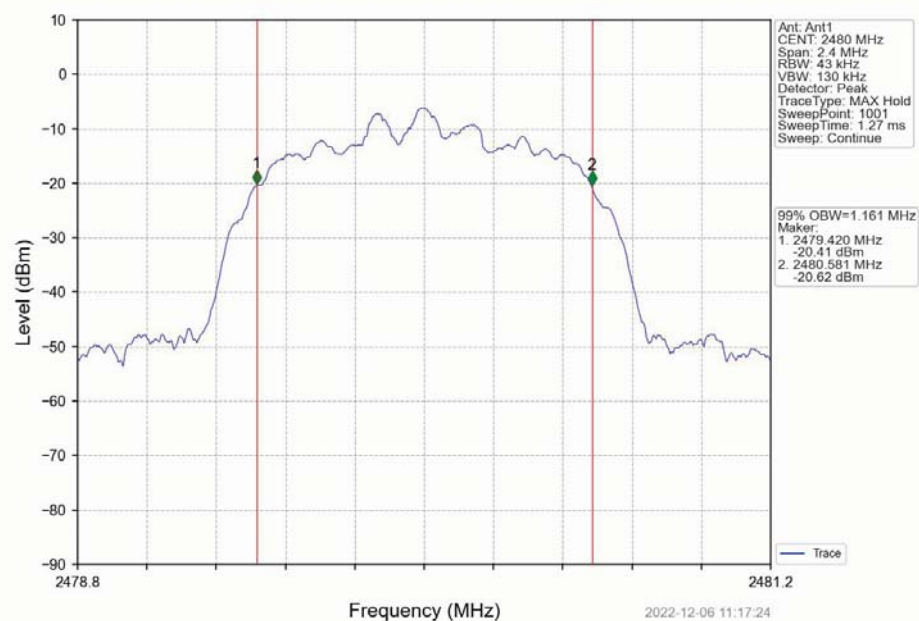
Pi/4DQPSK_2DH5_HCH_2480MHz_Ant1_NTNV
