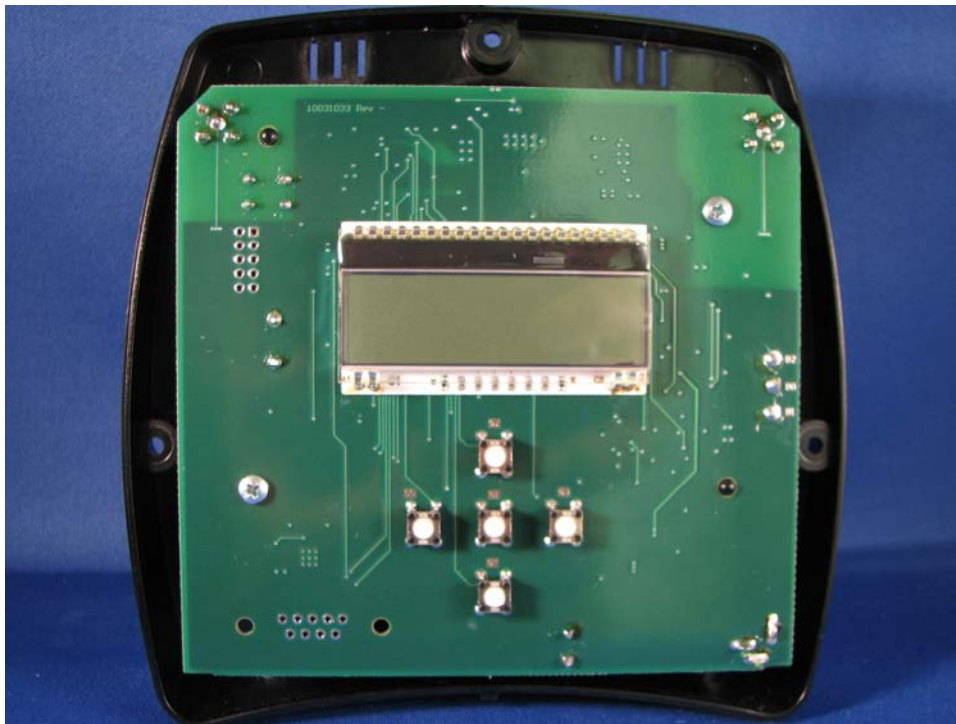
Front of Board
