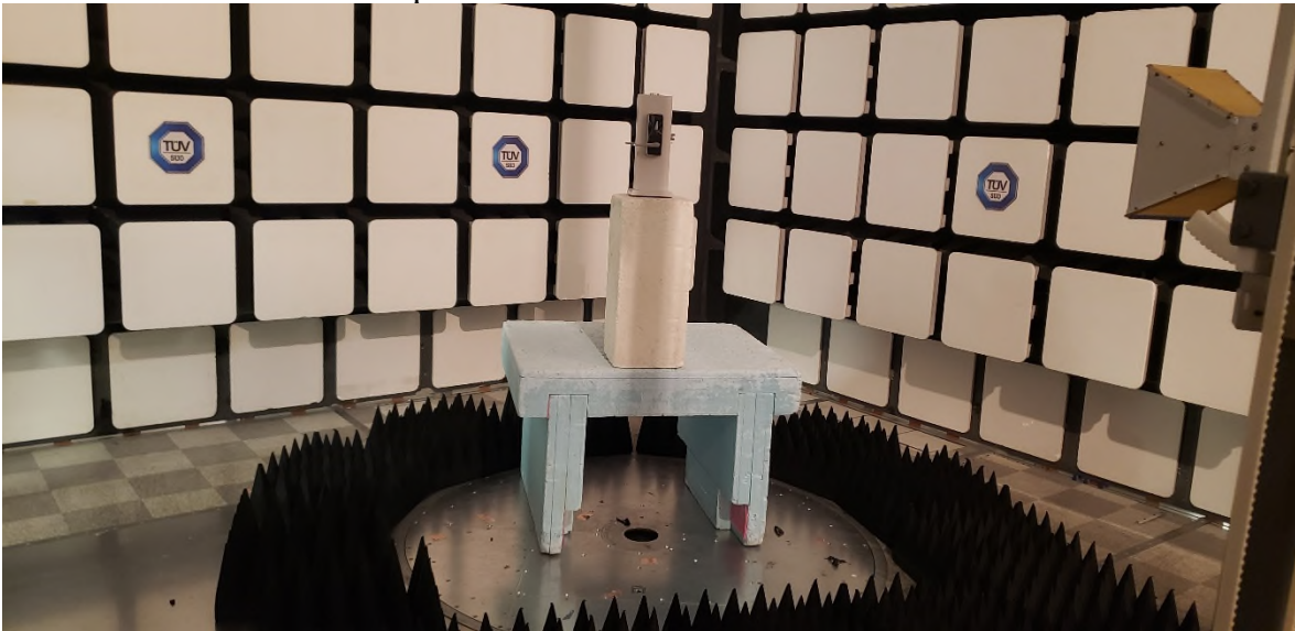
Radiated Emissions 1 GHz to 18 GHz – Test setup
