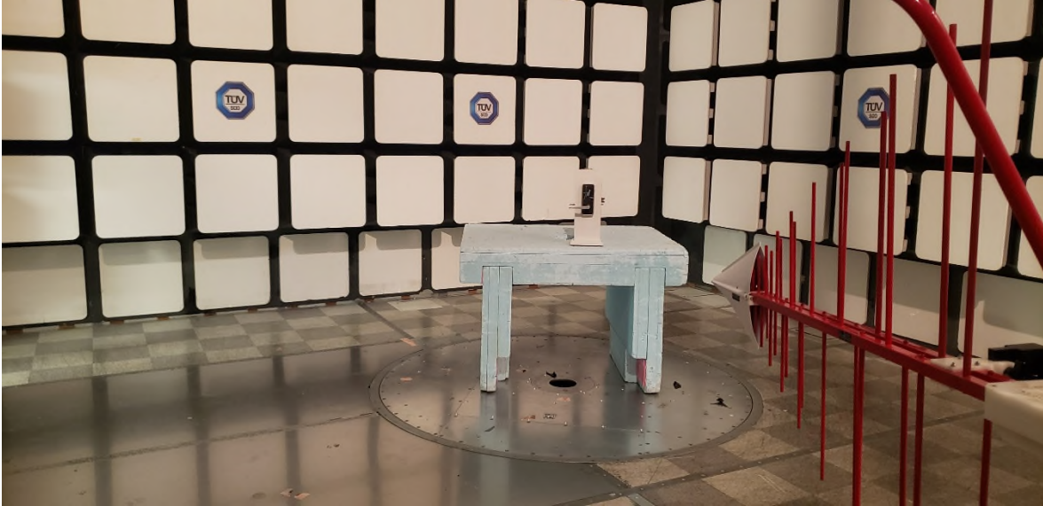
30 MHz to 1 GHz – Test setup
