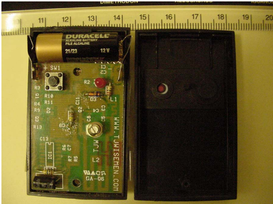
Inside with front cover removed, shown at right
