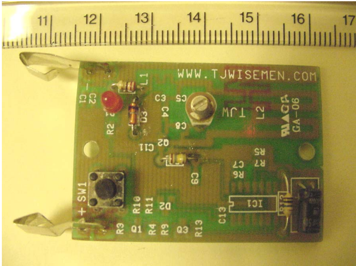
PCB Front
