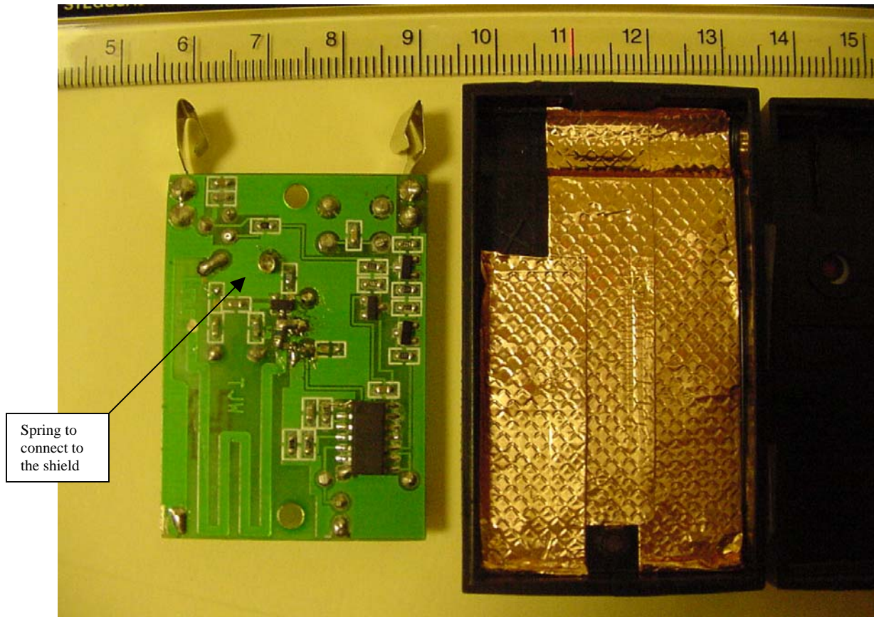
Interior rear of pcb removed from housing, shielding on the inside of the rear housing shown at right.
