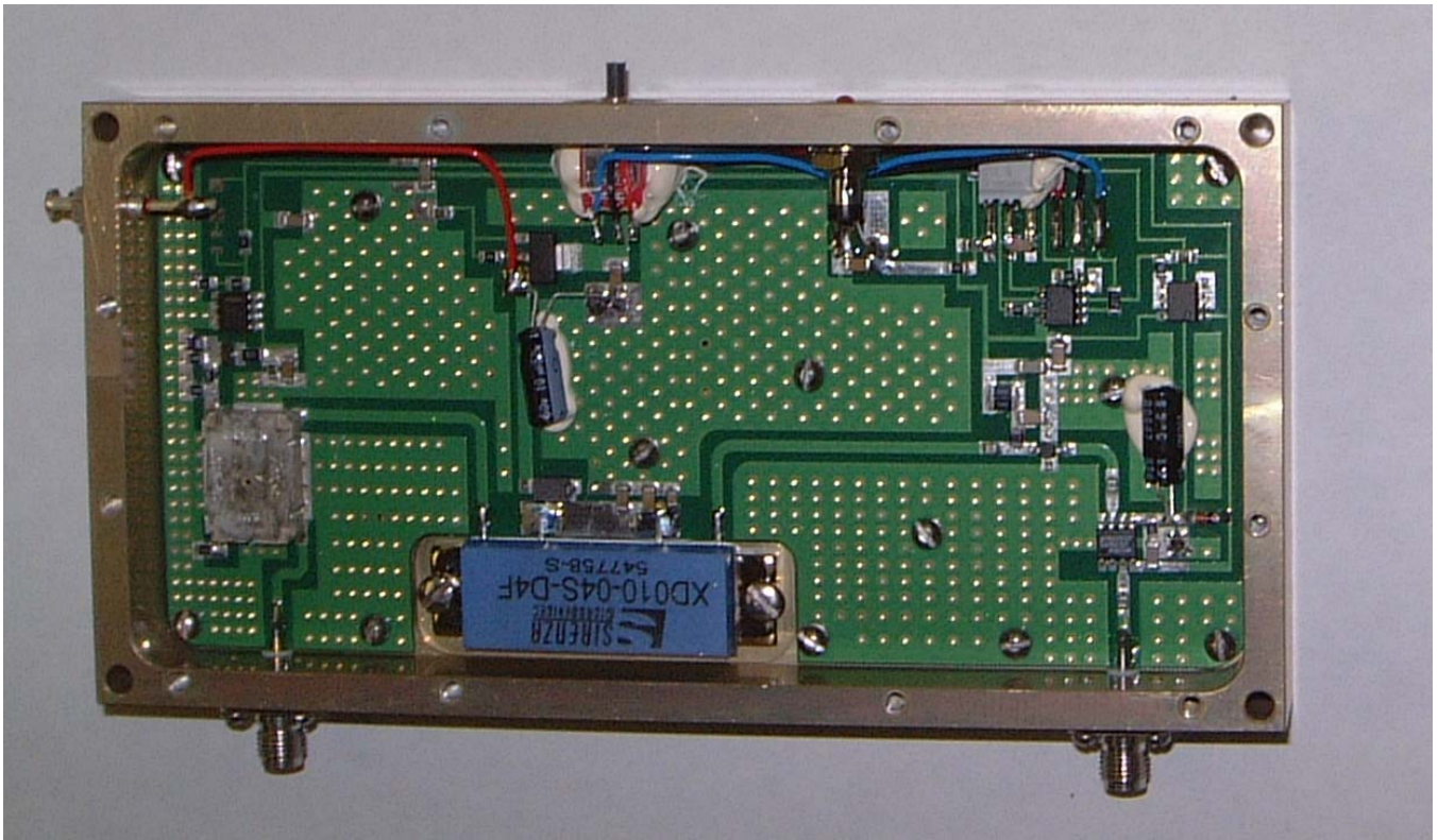
Power Amplifier for Uplink Front View in Housing
