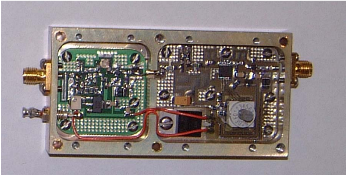
Low Noise Amplifier/Pre-Amplifier for Downlink Front View in Housing
