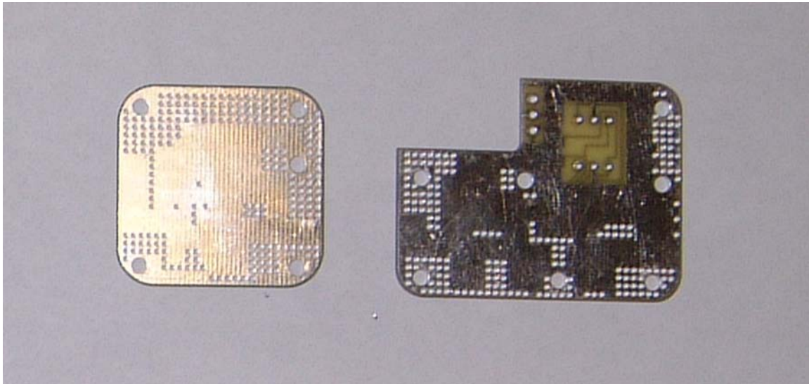
Low Noise Amplifier/Pre-Amplifier for Downlink Back View
