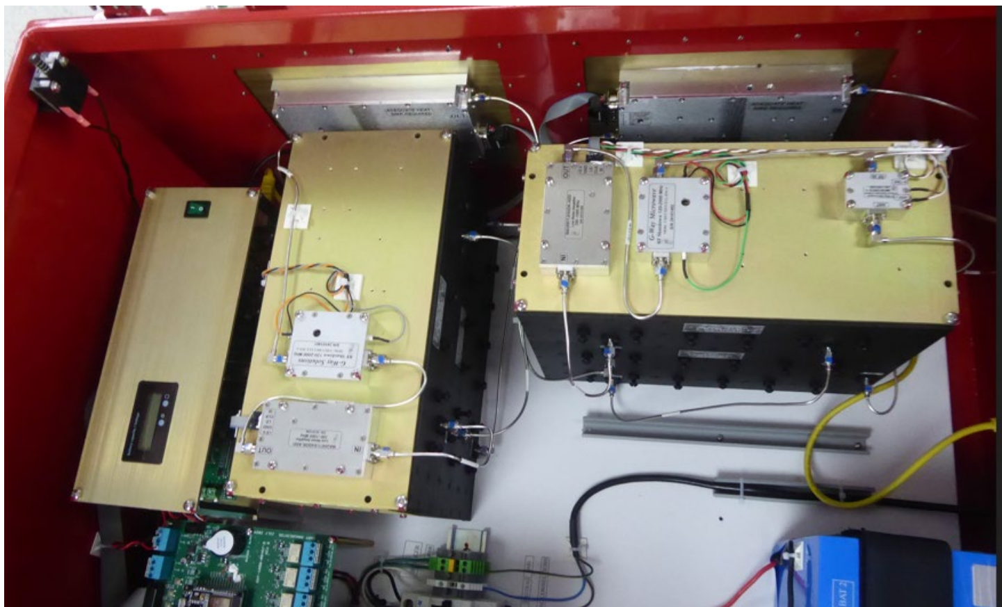
G-Wave 1-BOX™ UHF Internal Photos: (cont)
