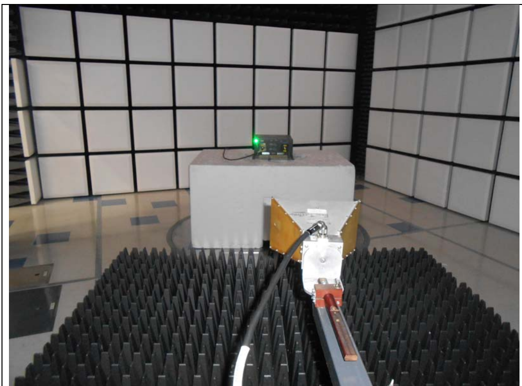
RF Radiated_above 1 GHz AB Enclosure
