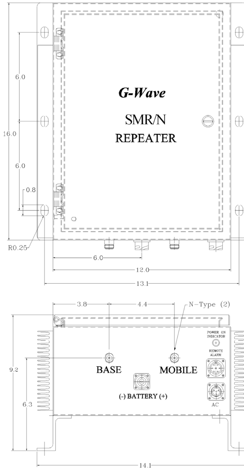
Figure 3: Mechanical Outline
