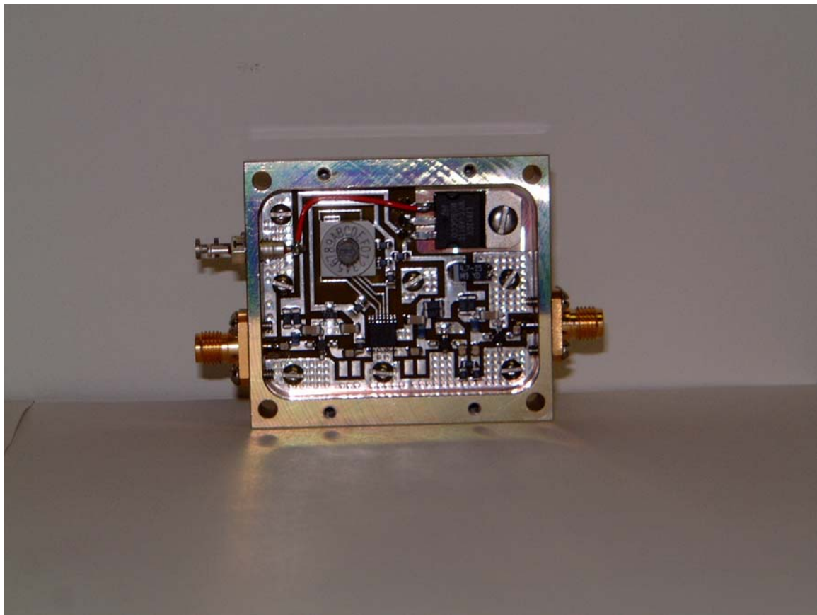
Uplink & Downlink LNA/Pre-Amp
