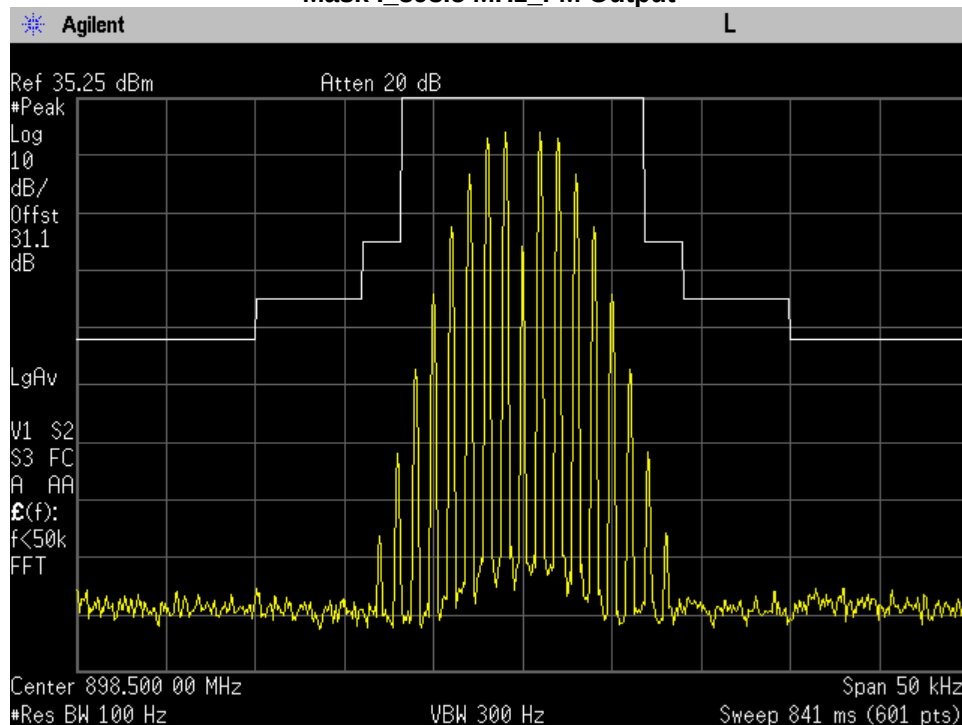
Mask I_898.5 MHz_FM Output
