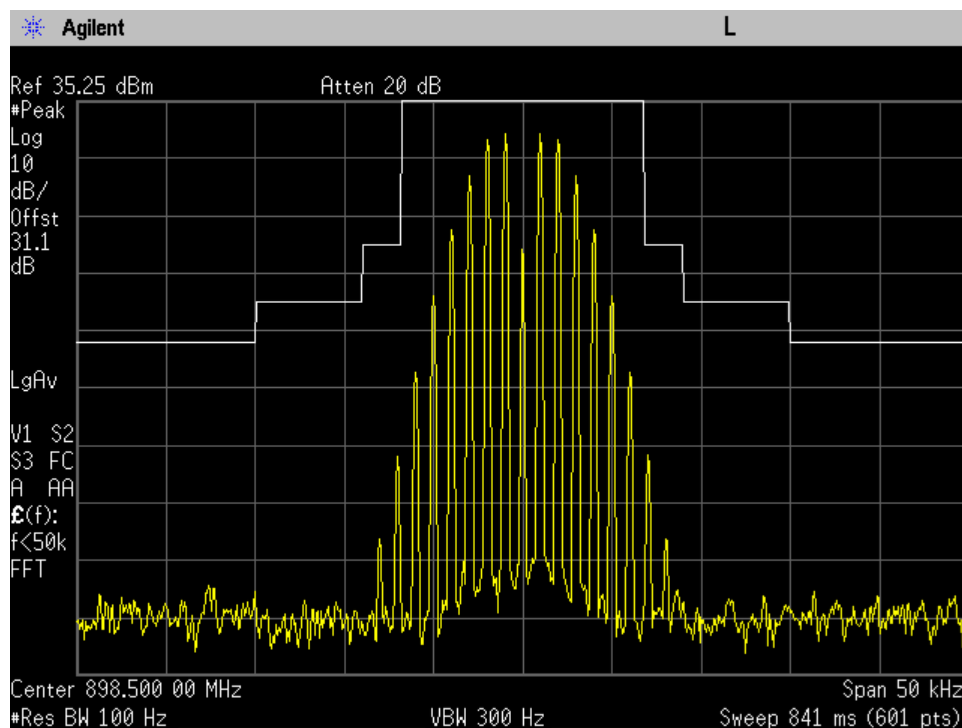
Mask I_898.5 MHz_FM Output_Pin + 3 dB
