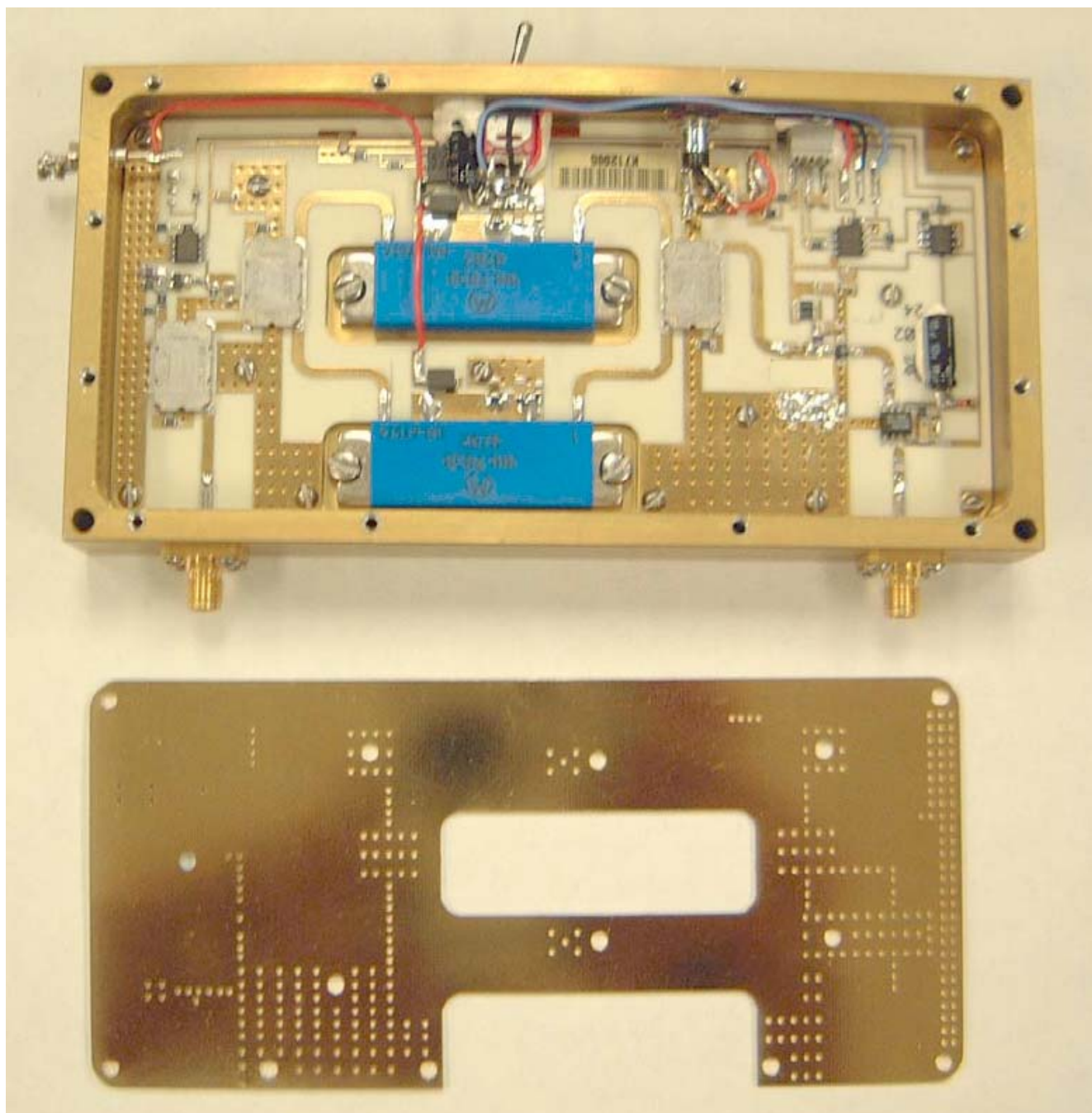
Downlink PA
