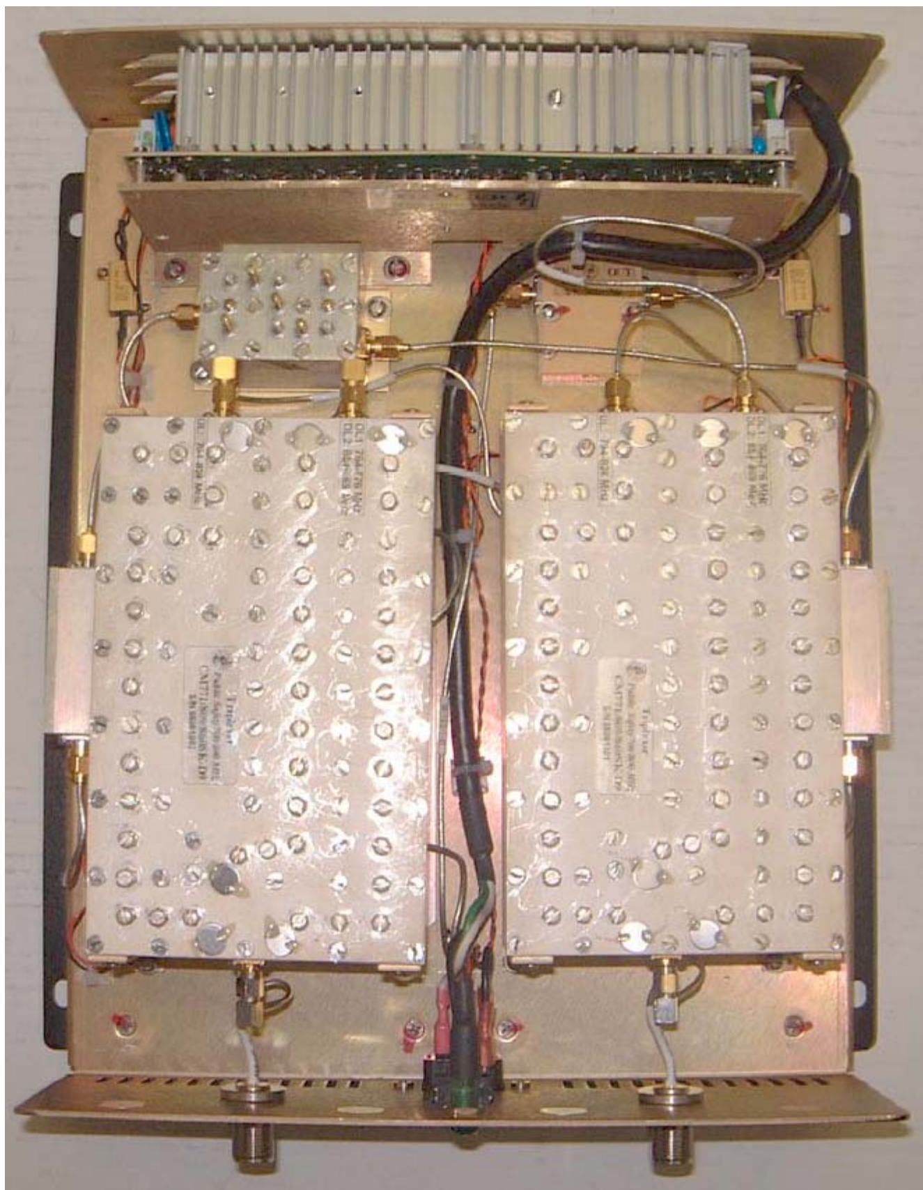
G-Wave Inc. Dual Band Bi-Directional Amplifier, Model BDA-PS7/PS8-2/10W-80-A FCC ID: Q8KPS7PS810W80
