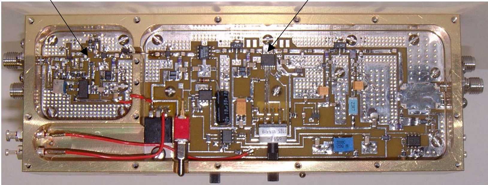
PCB Front final assembly (same assemblies for uplink and downlink)
