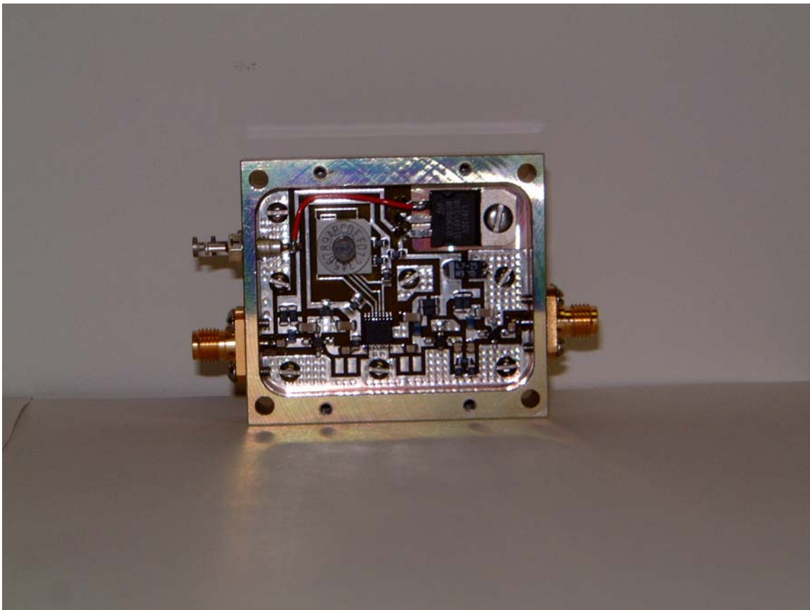
Uplink & Downlink LNA/Pre-Amp Front
