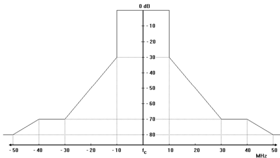
Figure 5: Transmitter power spectrum mask
