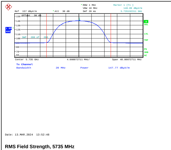
RMS Field Strength, 5735 MHz
