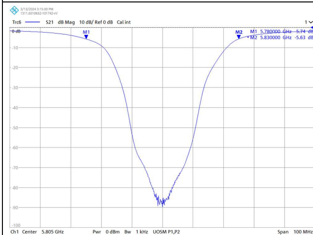
Filter response, 5805 MHz
