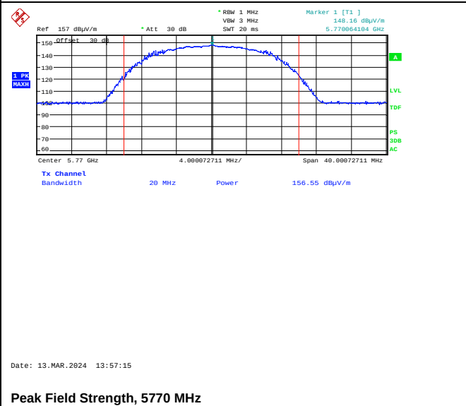
Peak Field Strength, 5770 MHz
