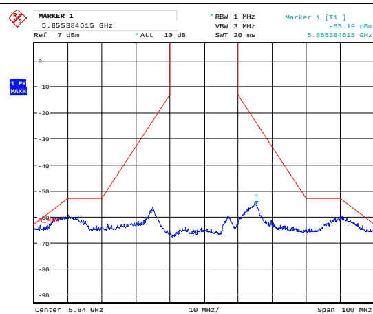
Carrier with Filter, 5840 MHz
