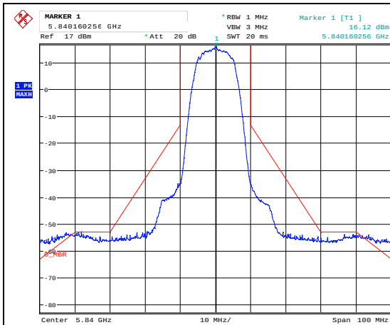
Spectrum Mask, 5840 MHz
