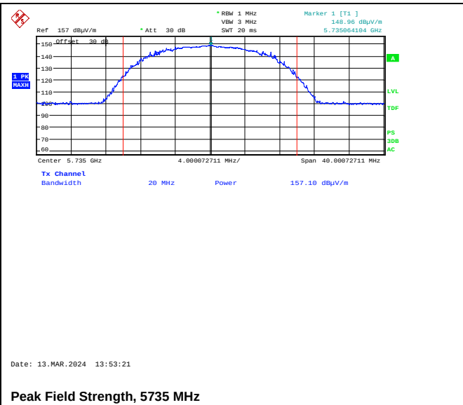
Peak Field Strength, 5735 MHz
