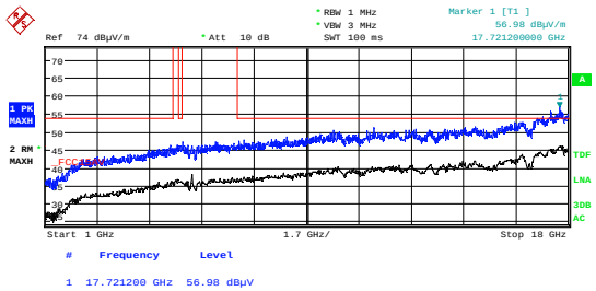
Radiated Emissions 1-18 GHz, 5735 MHz, HP
