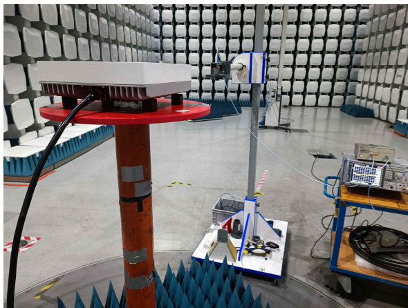
Pre-scan 18 – 40 GHz
