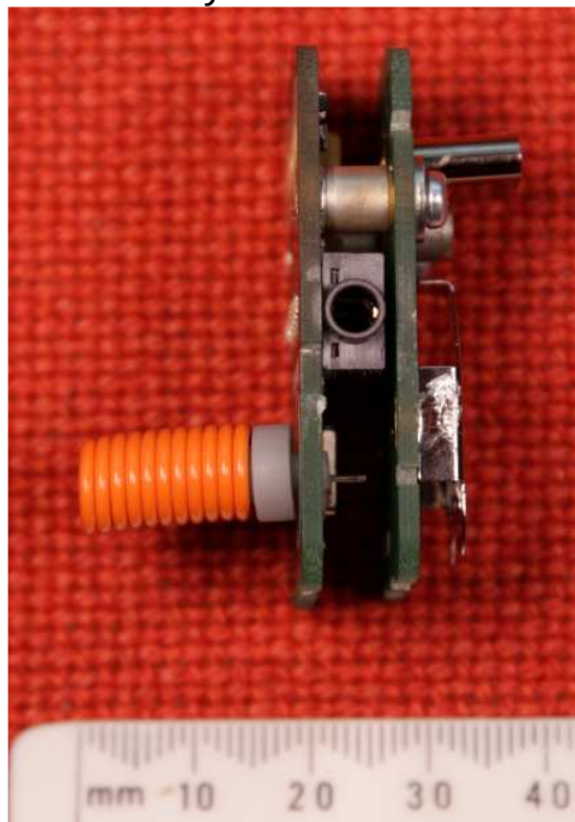
PC06878 Internal Assembly with Ariel and Moulding- Side angle
