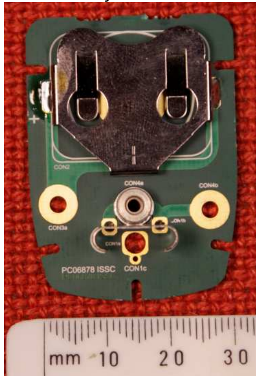
PC06878 Battery Plate Section Bottom
