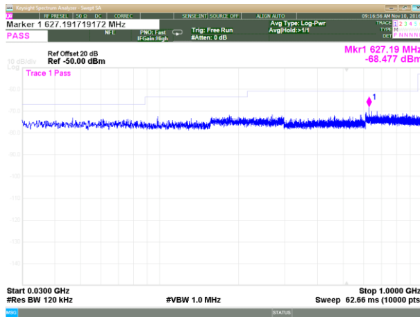
Plot 3.5.65 Emissions in restricted frequency bands test results, Conducted measurements, 30 MHz – 1000 MHz, F_c = 2440 MHz, BW = 8.4 MHz, Bit Rate = 8 Mbps
