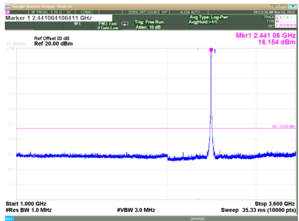
Plot 3.5.66 Emissions in restricted frequency bands test results, Conducted measurements, 1 GHz – 3.6 GHz, F_c = 2440 MHz, BW = 8.4 MHz, Bit Rate = 8 Mbps
