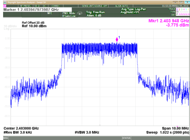
Plot 3.3.4 Maximum Power Spectral Density test results, F_c = 2403\text{MHz} , BW = 4.2\text{ MHz} , Bit Rate = 4 Mbps
