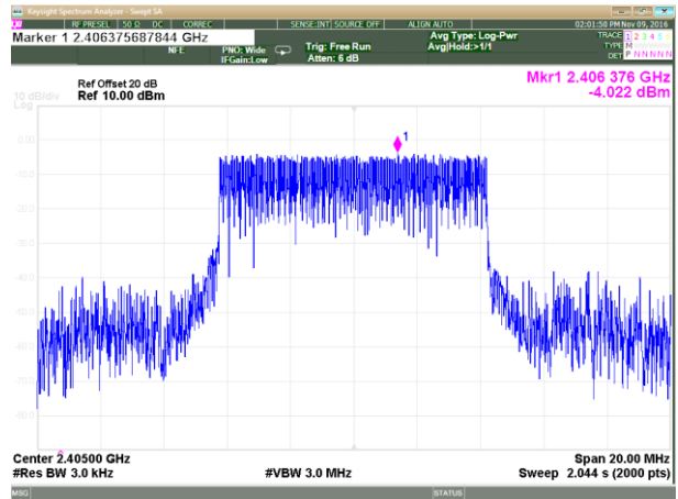
Plot 3.3.7 Maximum Power Spectral Density test results, F_c = 2405\text{MHz} , BW = 8.4\text{ MHz} , Bit Rate = 6.4 Mbps
