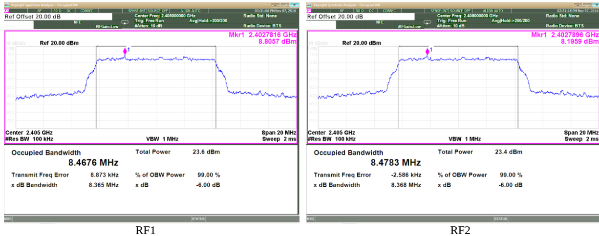
Plot 3.1.7 6 dB DTS Bandwidth, BW = 8.4 MHz, Bit rate = 6.4 Mbps, Fc = 2405 MHz
