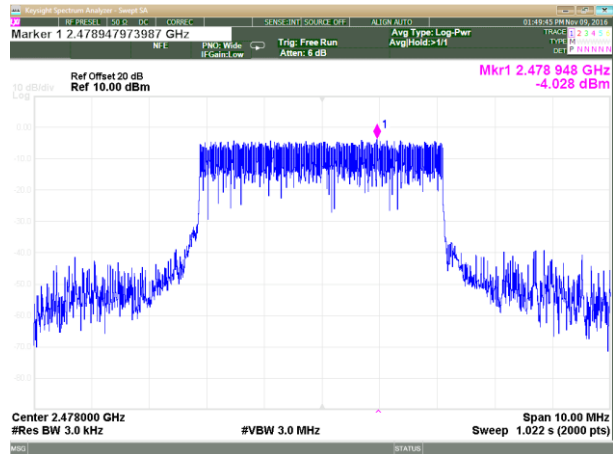
Plot 3.3.3 Maximum Power Spectral Density test results, F_c = 2478\text{MHz} , BW = 4.2\text{ MHz} , Bit Rate = 1.6 Mbps
