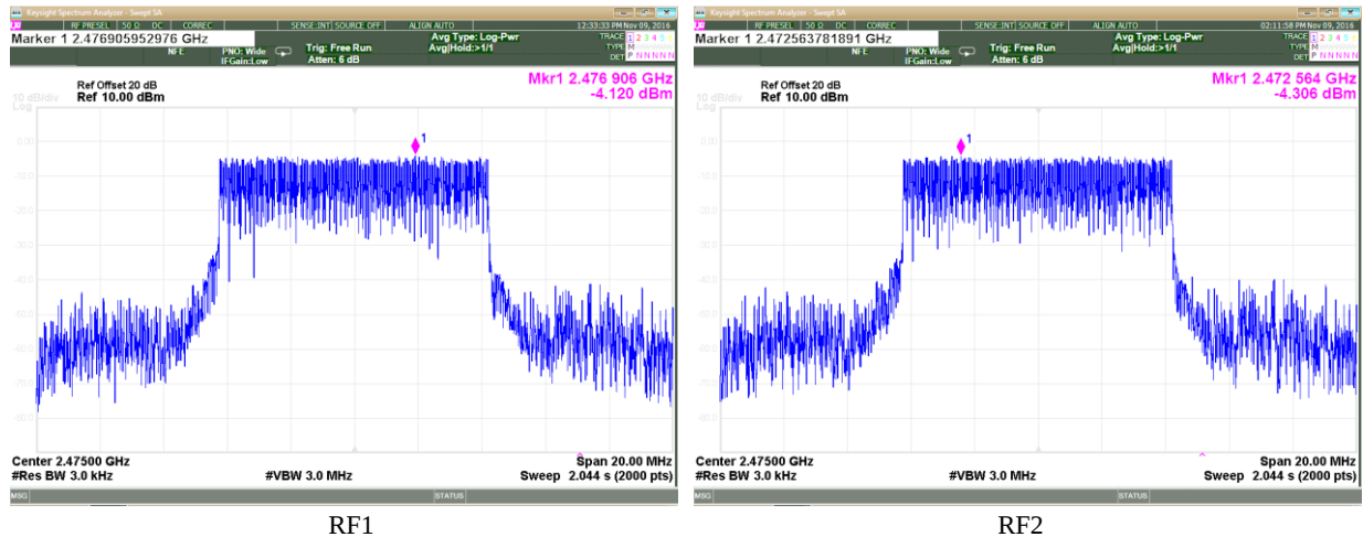
Plot 3.3.12 Maximum Power Spectral Density test results, F_c = 2475\text{MHz} , BW = 8.4\text{ MHz} , Bit Rate = 8 Mbps
