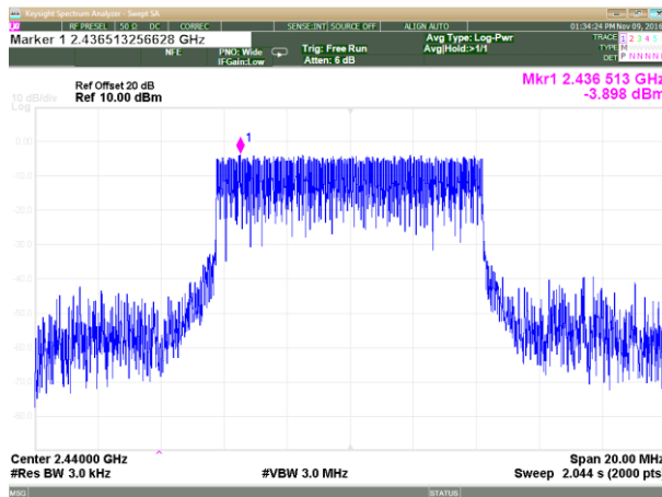
Plot 3.3.8 Maximum Power Spectral Density test results, F_c = 2440\text{MHz} , BW = 8.4\text{ MHz} , Bit Rate = 6.4 Mbps
