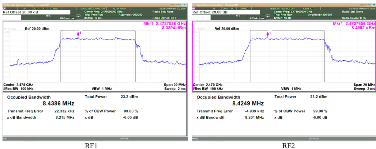
Plot 3.1.12 6 dB DTS Bandwidth, BW = 8.4 MHz, Bit rate = 8.0 Mbps, Fc = 2475 MHz
