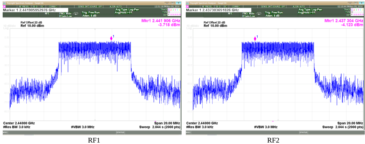
Plot 3.3.11 Maximum Power Spectral Density test results, F_c = 2440\text{MHz} , BW = 8.4\text{ MHz} , Bit Rate = 8 Mbps
