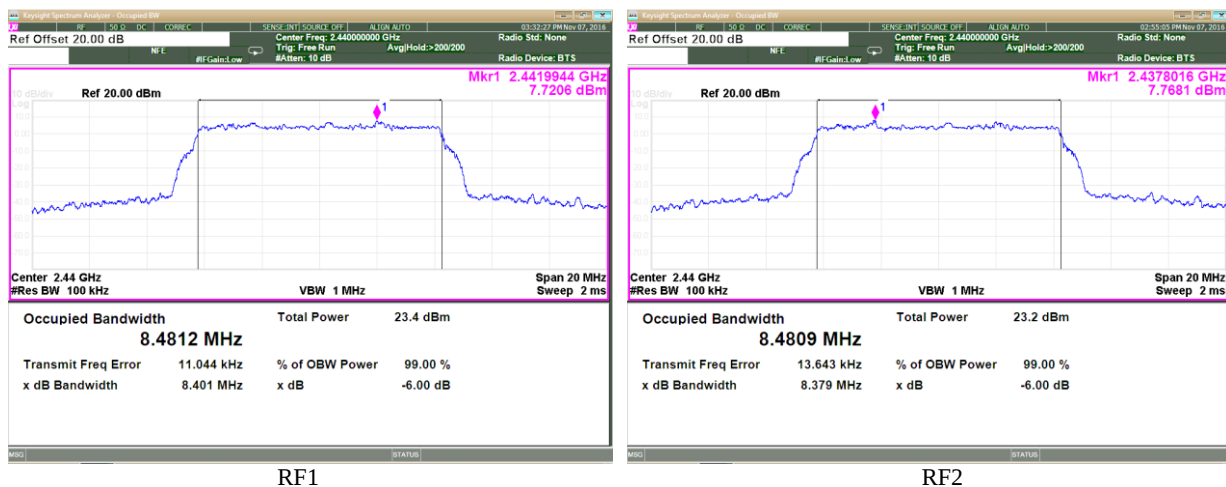
Plot 3.1.8 6 dB DTS Bandwidth, BW = 8.4 MHz, Bit rate = 6.4 Mbps, Fc = 2440 MHz
