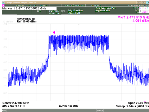
Plot 4.3.9 Maximum Power Spectral Density test results, F_c = 2475\text{MHz} , BW = 8.4\text{ MHz} , Bit Rate = 6.4 Mbps
