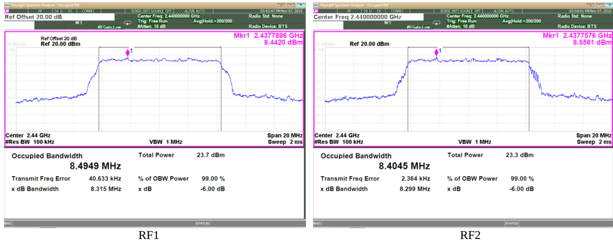
Plot 3.1.11 6 dB DTS Bandwidth, BW = 8.4 MHz, Bit rate = 8.0 Mbps, Fc = 2440 MHz
