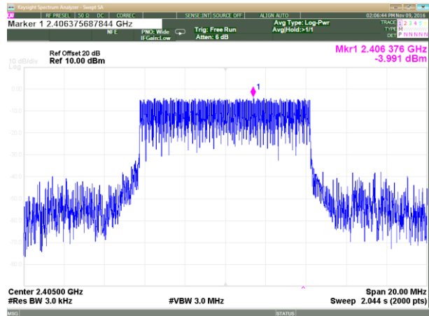
Plot 3.3.10 Maximum Power Spectral Density test results, F_c = 2405\text{MHz} , BW = 8.4\text{ MHz} , Bit Rate = 8 Mbps
