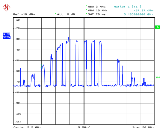
Waveform of EUT links up with Client
