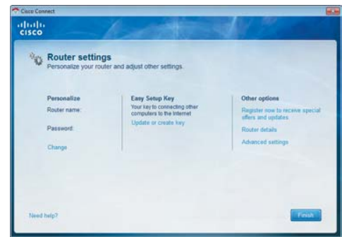
Router Settings
