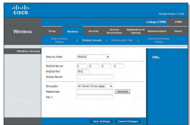
RADIUS
