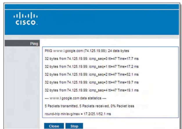
Diagnostics > Ping
