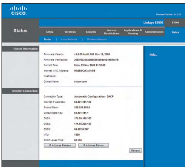
Status > Router
