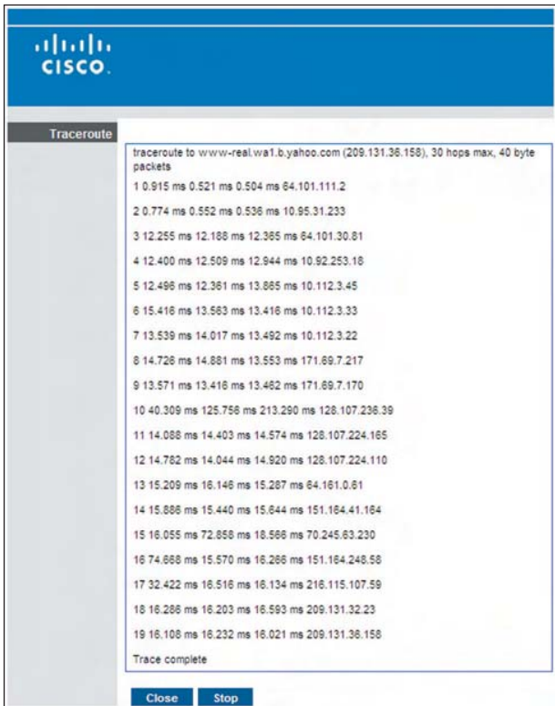
Diagnostics > Traceroute
