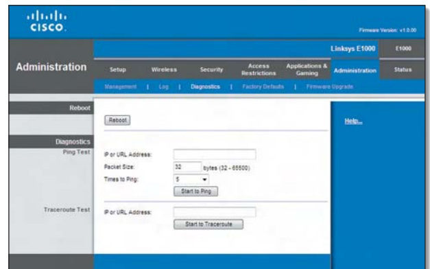
Administration > Diagnostics
