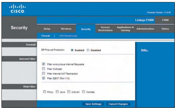
Security > Firewall
