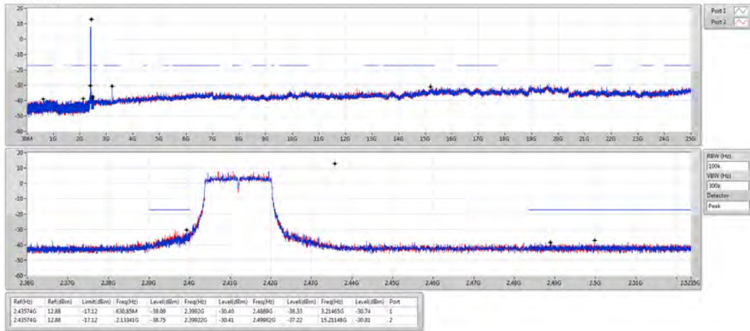
802.11g-BF_Nss1,(6Mbps)_2TX 2412MHz
