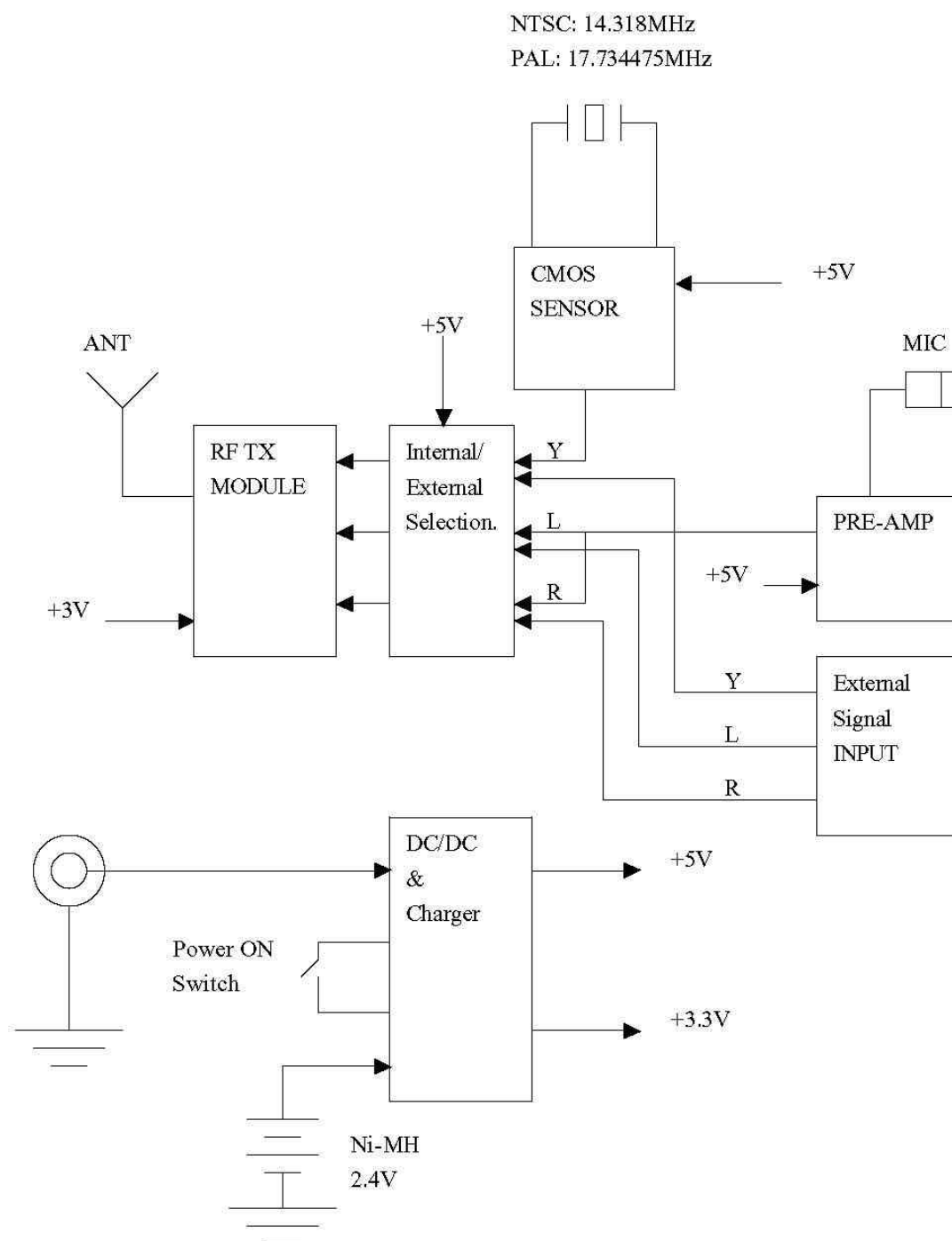
GA-251 TX BLOCK DIAGRAM
