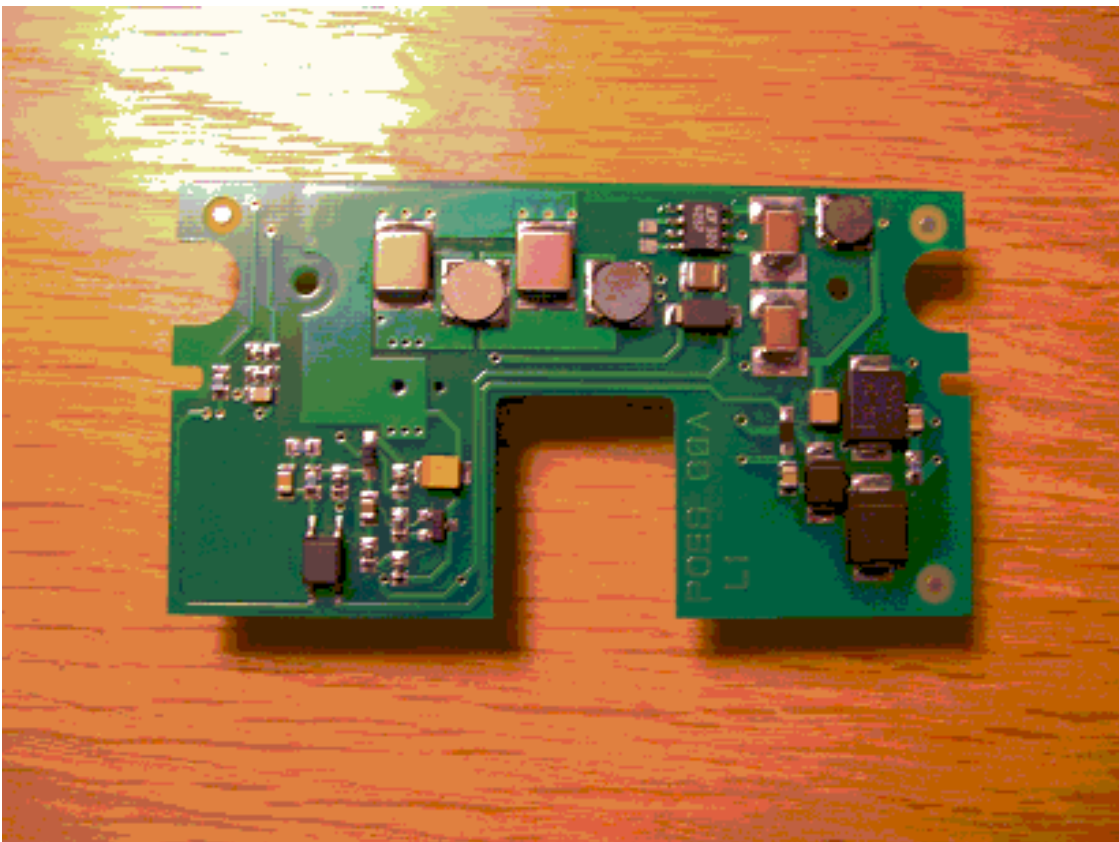
PoE Board front
