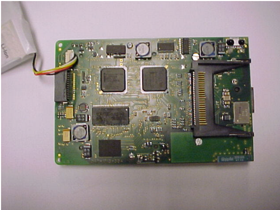
MainBoard front without battery
