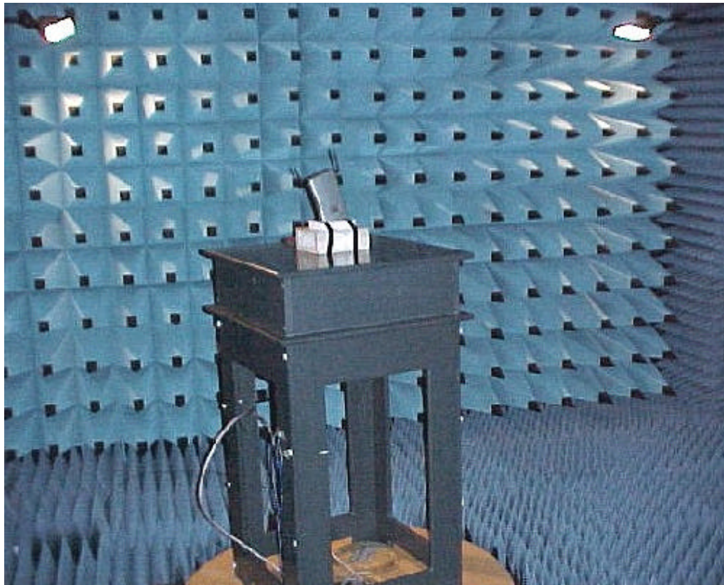
Test set-up 1-26 GHz
