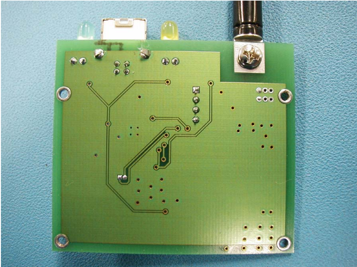
Figure 4 Bottom of main board with antenna
