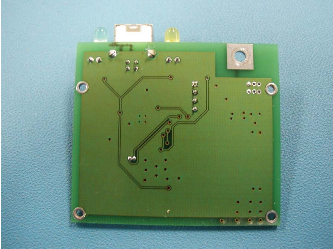
Figure 5 Bottom of main board without antenna
