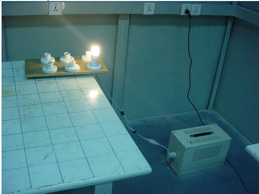
4.32 Photo of Power Line Conducted Emission Test (ZD17a-5W)
