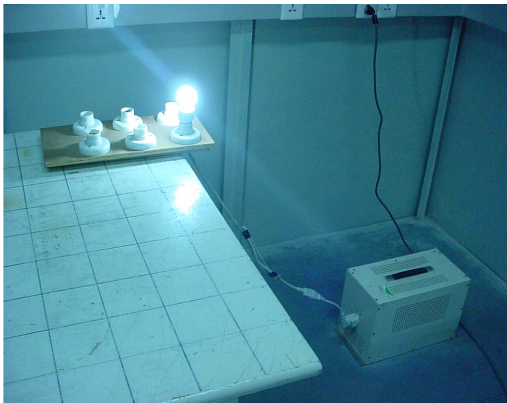
4.28 Photo of Power Line Conducted Emission Test (ZD16a-9W)
