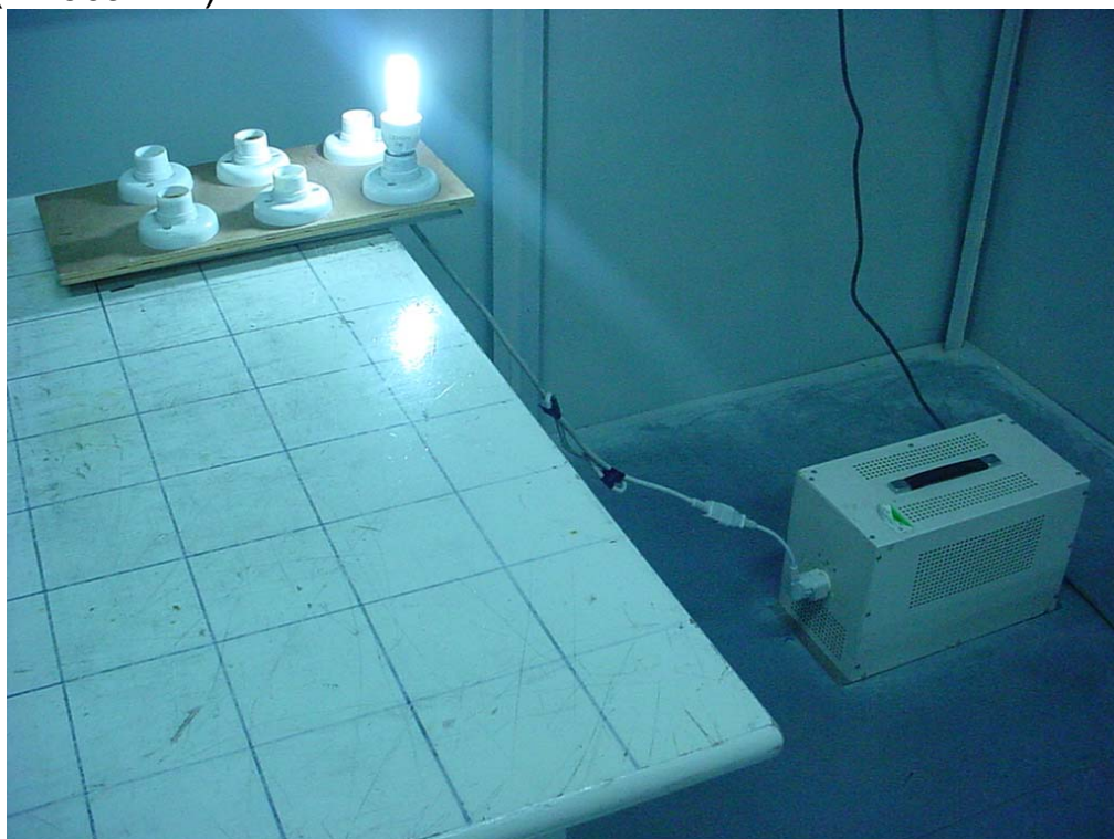
4.42 Photo of Power Line Conducted Emission Test (ZD06a-7W)
