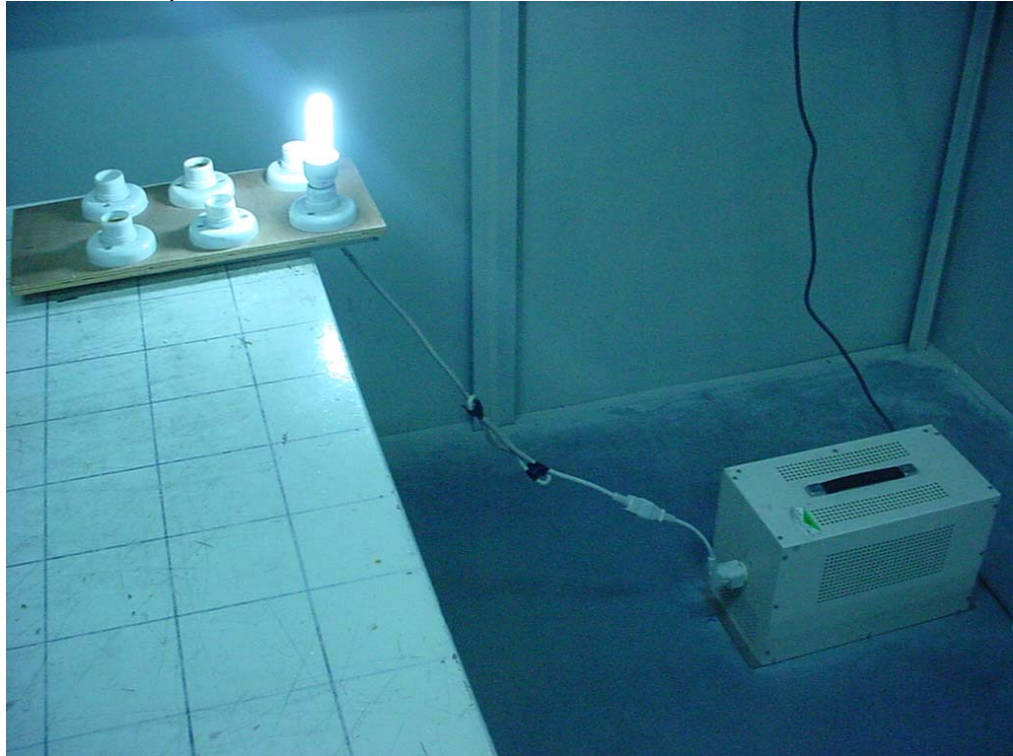
4.44 Photo of Power Line Conducted Emission Test (ZD06a-11W)
