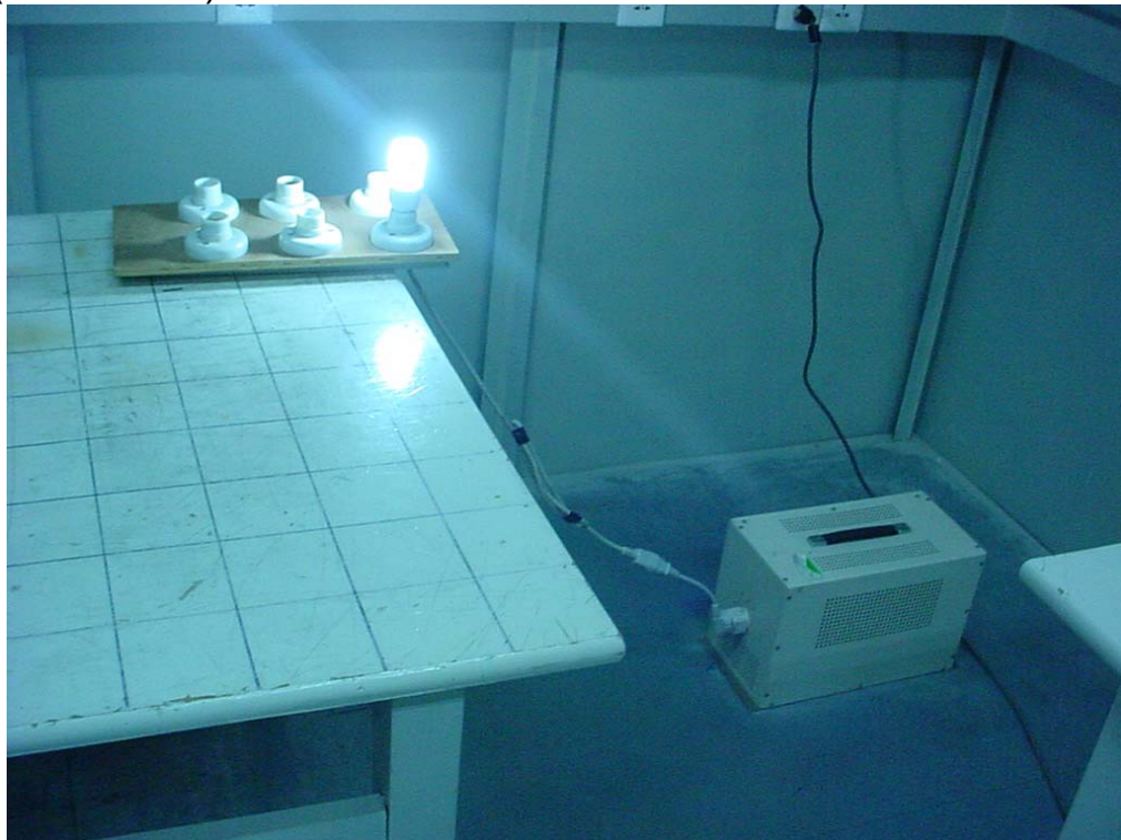
4.34 Photo of Power Line Conducted Emission Test (ZD17a-9W)
