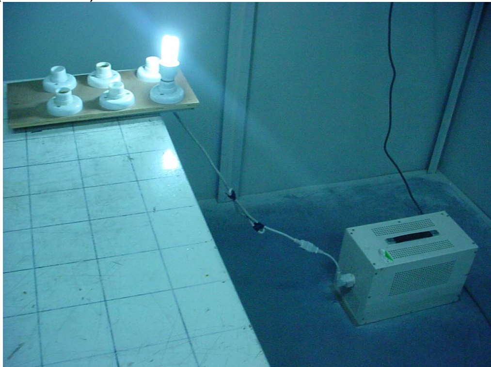
4.38 Photo of Power Line Conducted Emission Test (ZD02a-7W)
