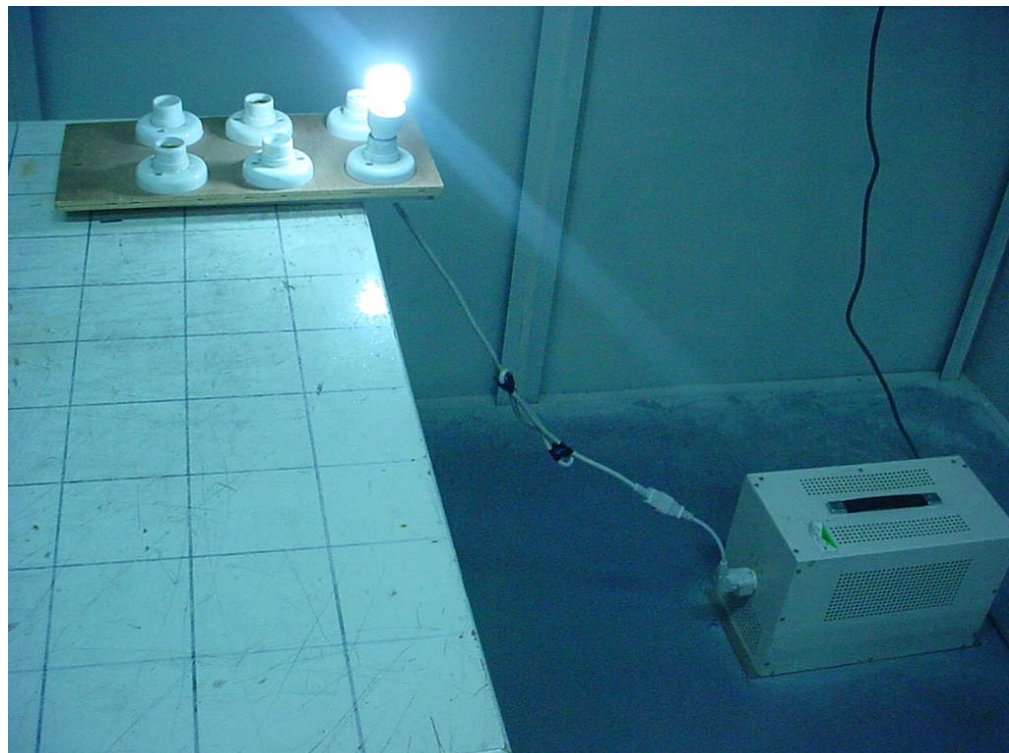
4.26 Photo of Power Line Conducted Emission Test (ZD16a-5W)
