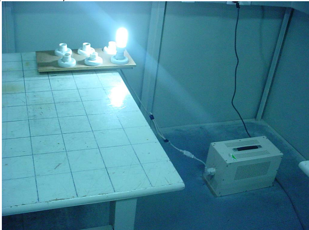
4.36 Photo of Power Line Conducted Emission Test (ZD17a-13W)
