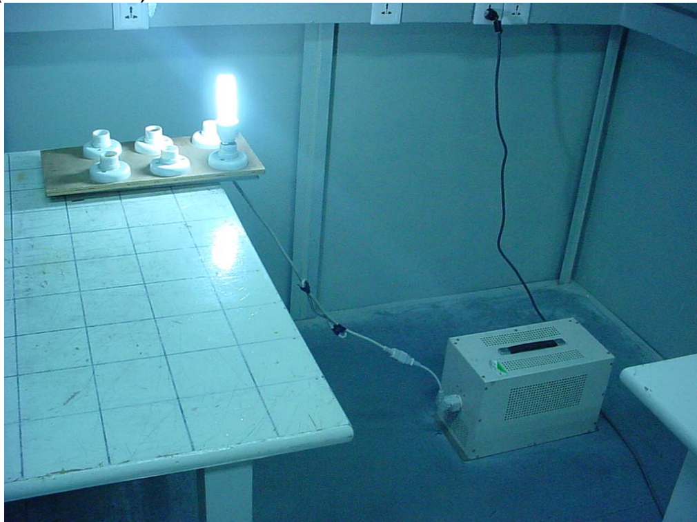
4.40 Photo of Power Line Conducted Emission Test (ZD02a-11W)
