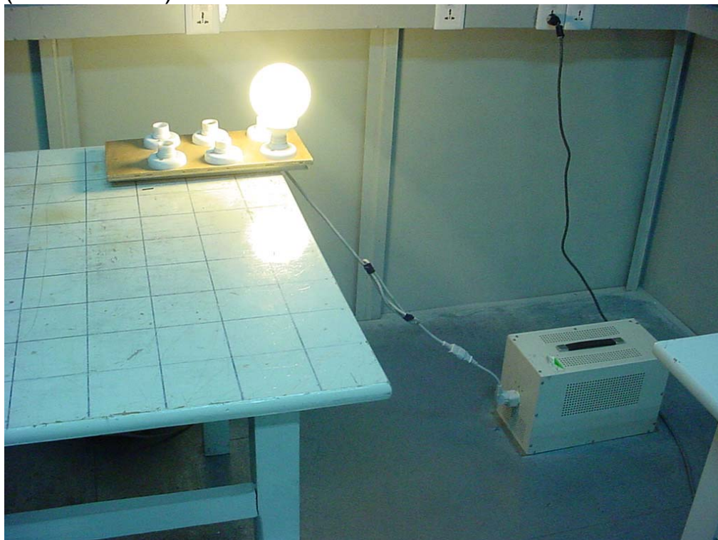
4.10 Photo of Power Line Conducted Emission Test (ZDFGa-23W)
