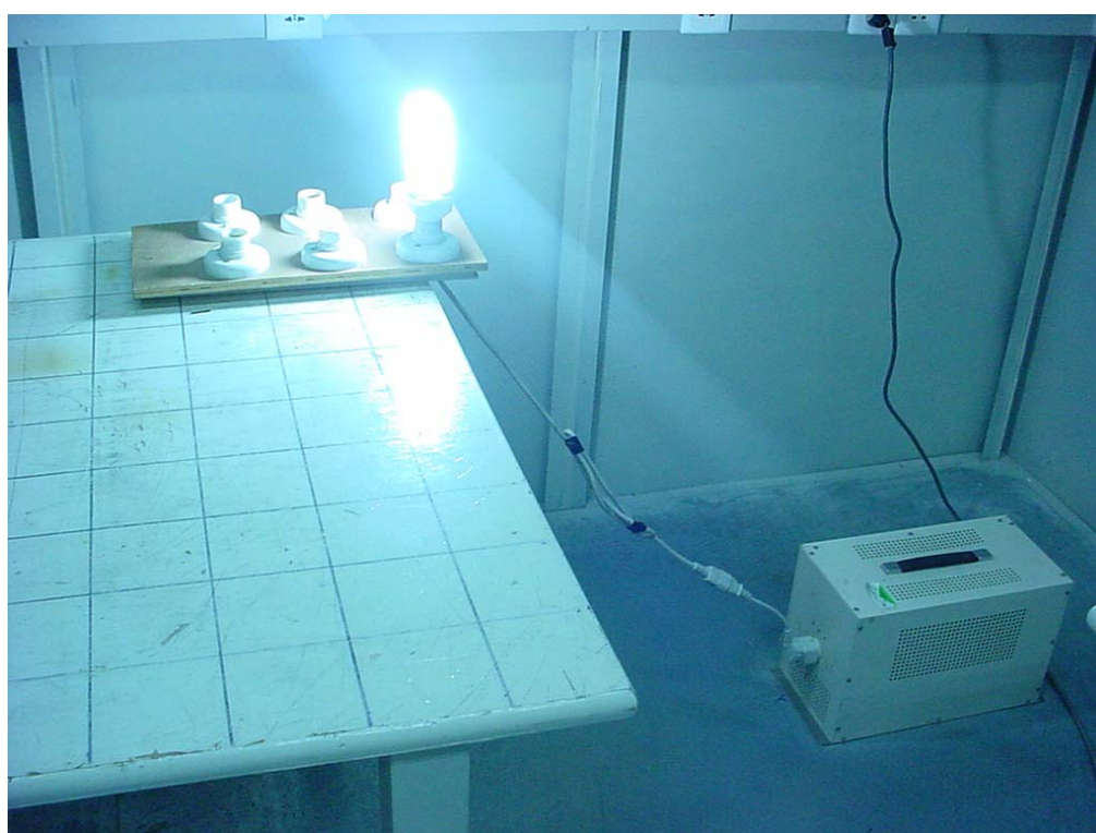
4.16 Photo of Power Line Conducted Emission Test (ZD04Aa-15W)
