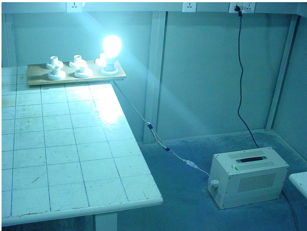
4.22 Photo of Power Line Conducted Emission Test (ZD04a-18W)
