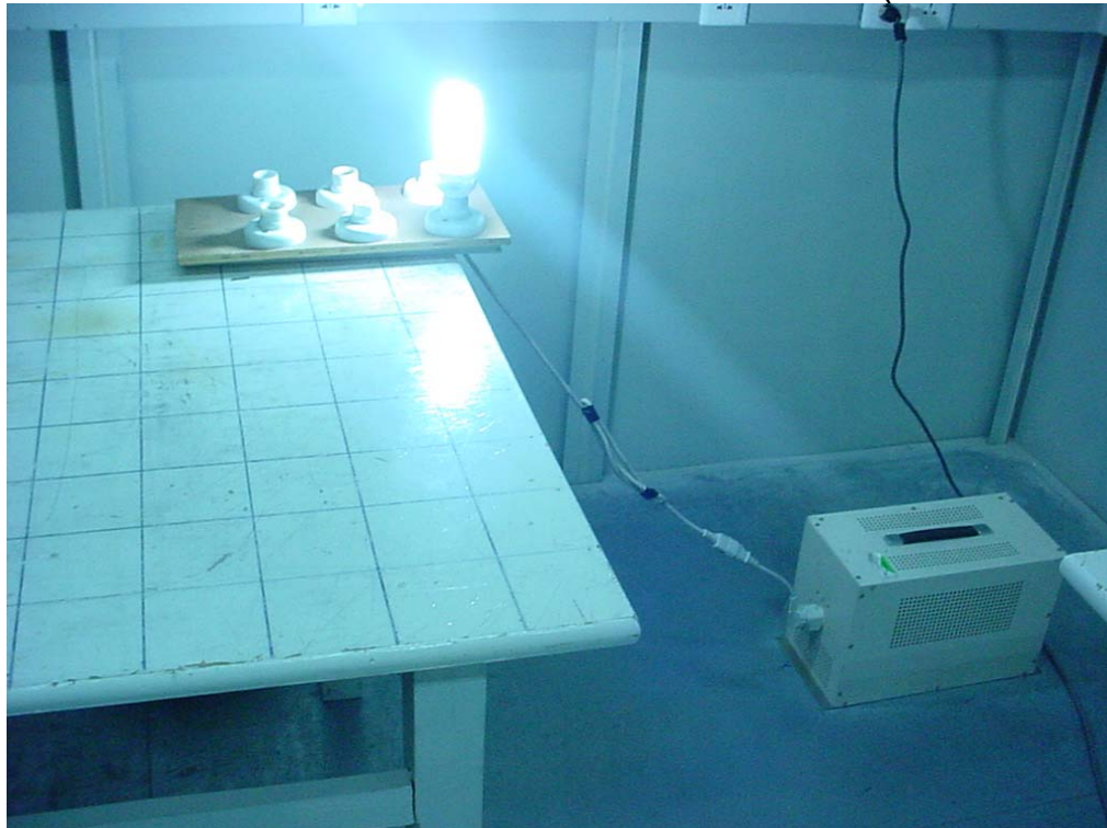
4.14 Photo of Power Line Conducted Emission Test (ZD07a-23W)
