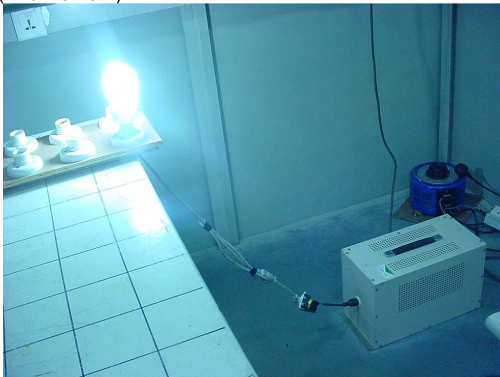
4.20 Photo of Power Line Conducted Emission Test (ZD04Aa-25W)
