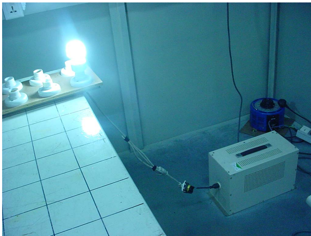
4.15 Photo of Power Line Conducted Emission Test (ZD07a-25W)
