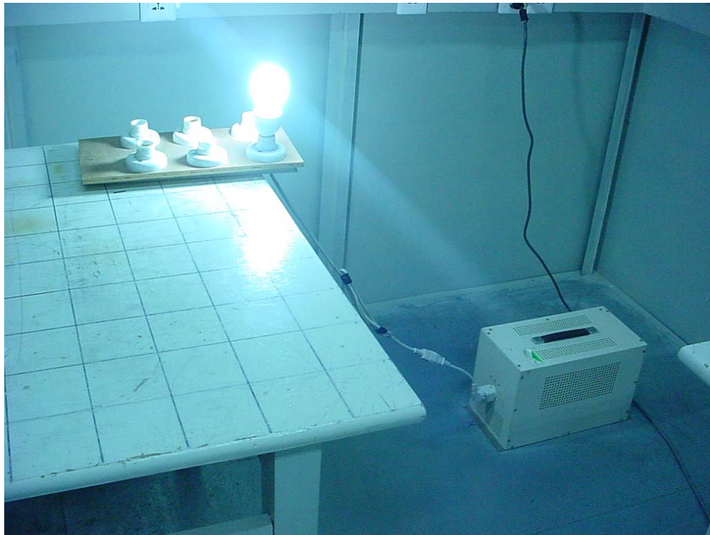
4.23 Photo of Power Line Conducted Emission Test (ZD04a-20W)
