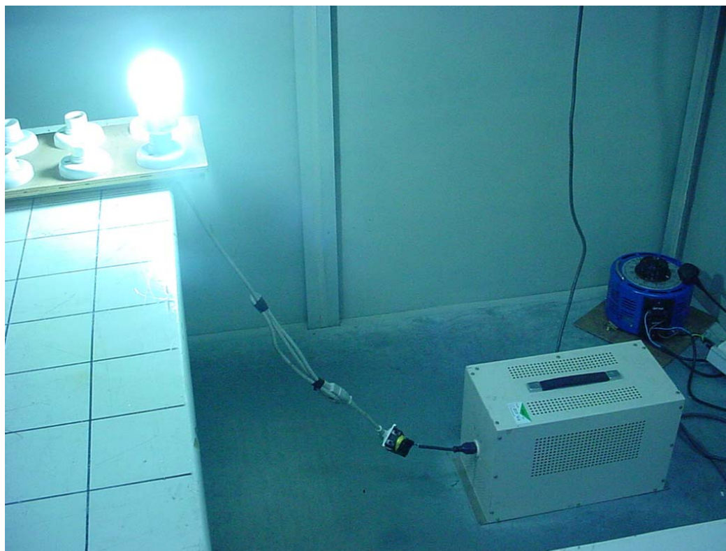
4.18 Photo of Power Line Conducted Emission Test (ZD04Aa-20W)
