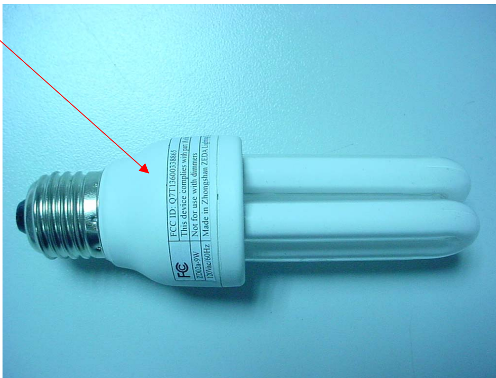
Figure 22 M/N: ZD02a-9W General Appearance
