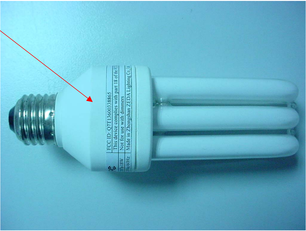
Figure 32 M/N: ZD07a-18W General Appearance
