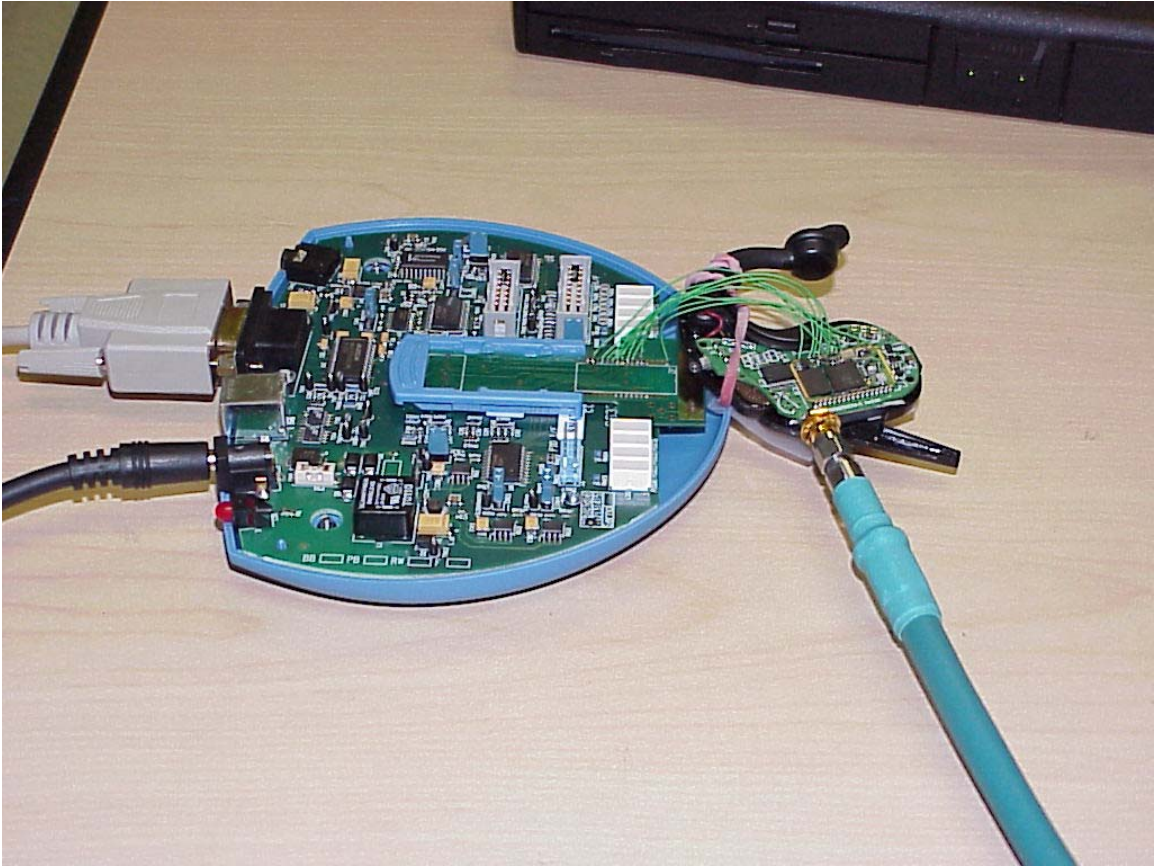
Test setup – Conducted measurements (showing EUT in test fixture)
