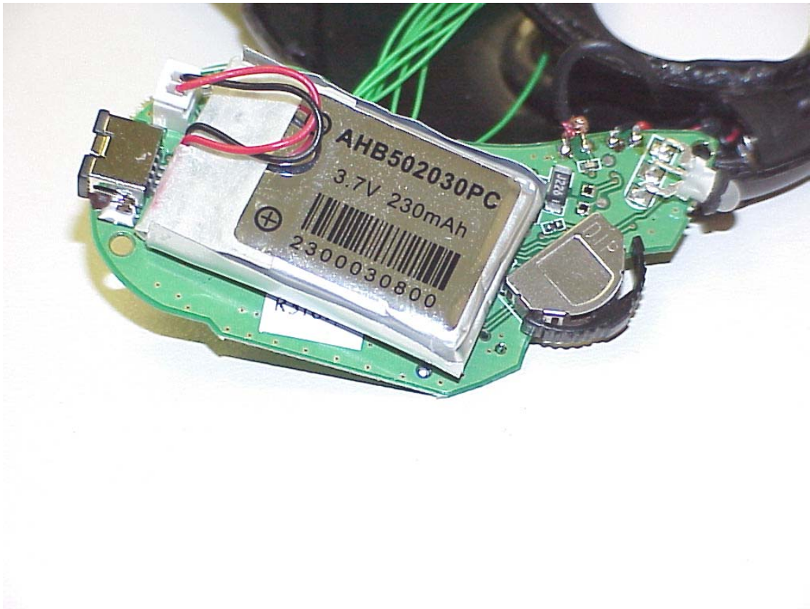
PCB – Bottom view
