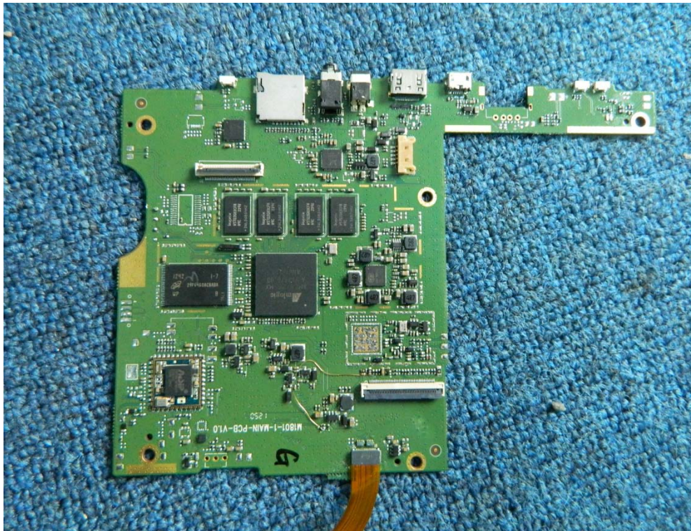
Mainboard (reverse)
