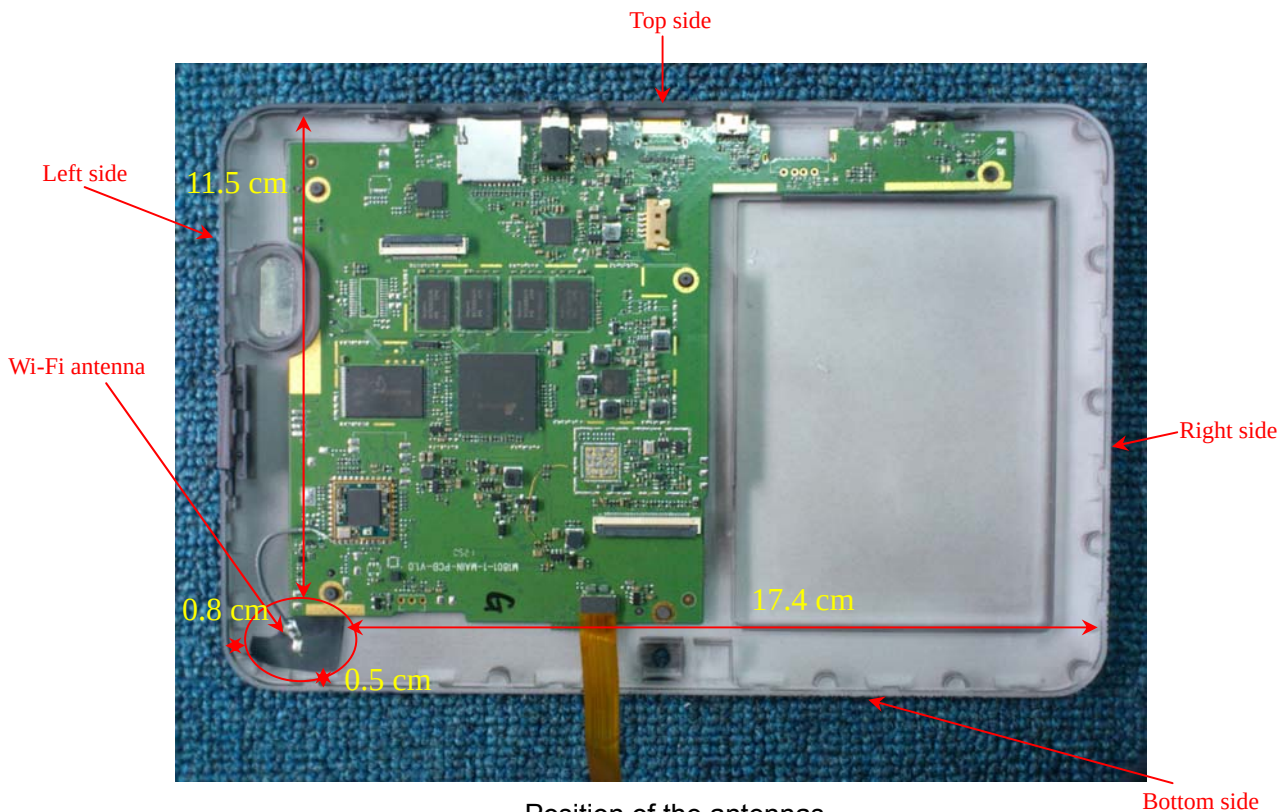
Position of the antennas
