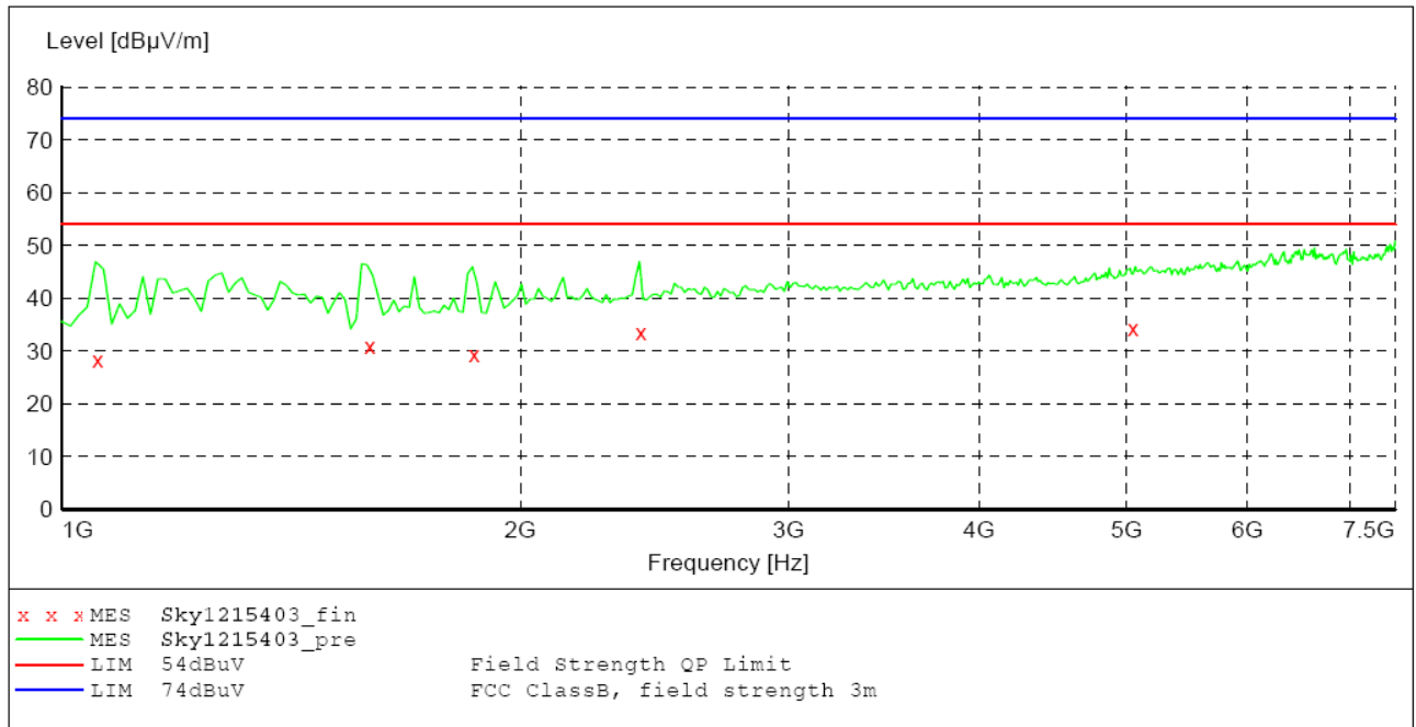
(Plot C: Test Antenna Horizontal 1G – 7.5G)
