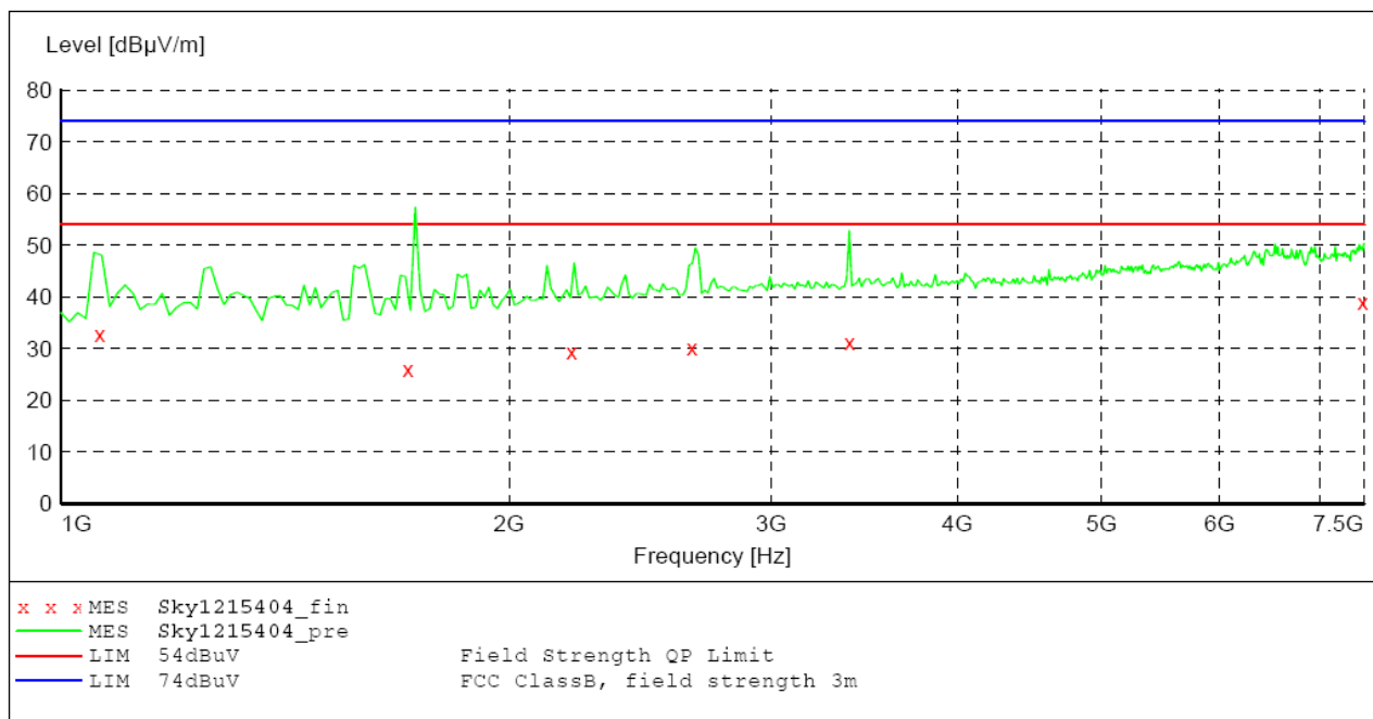
(Plot D: Test Antenna Vertical 1G – 7.5G)
