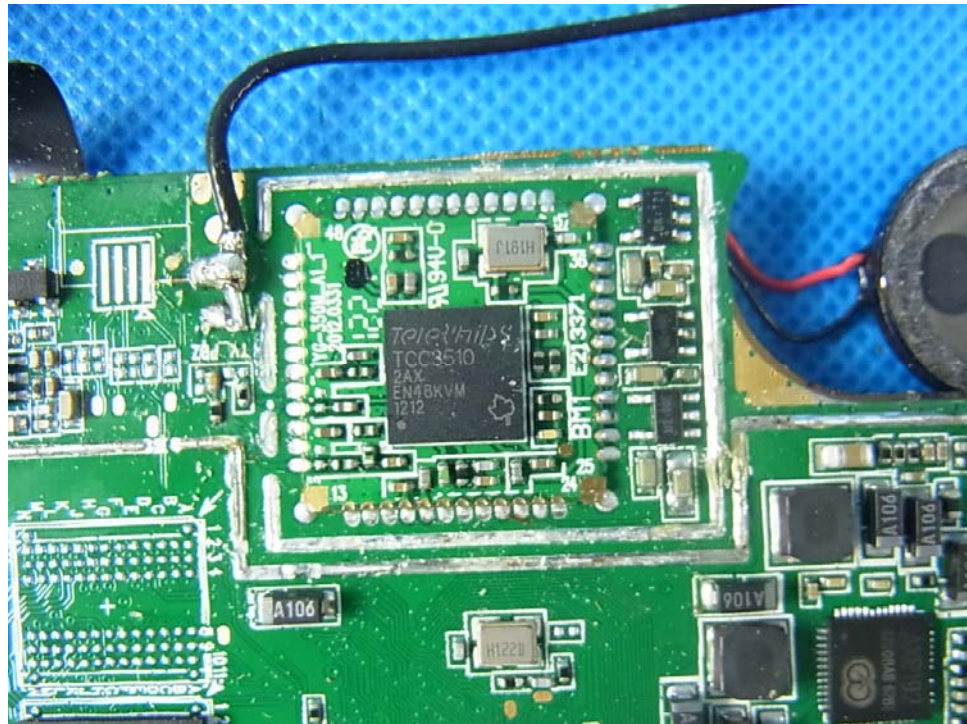
Photo 16 TV ANT
