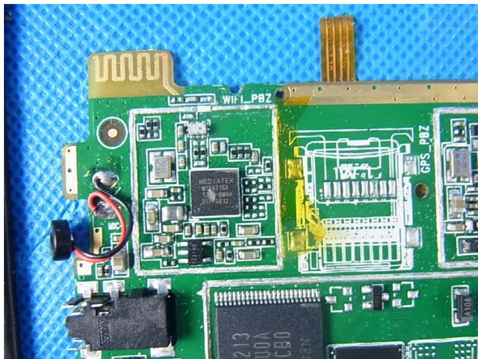
Photo 14 WIFI(PCB ANT)
