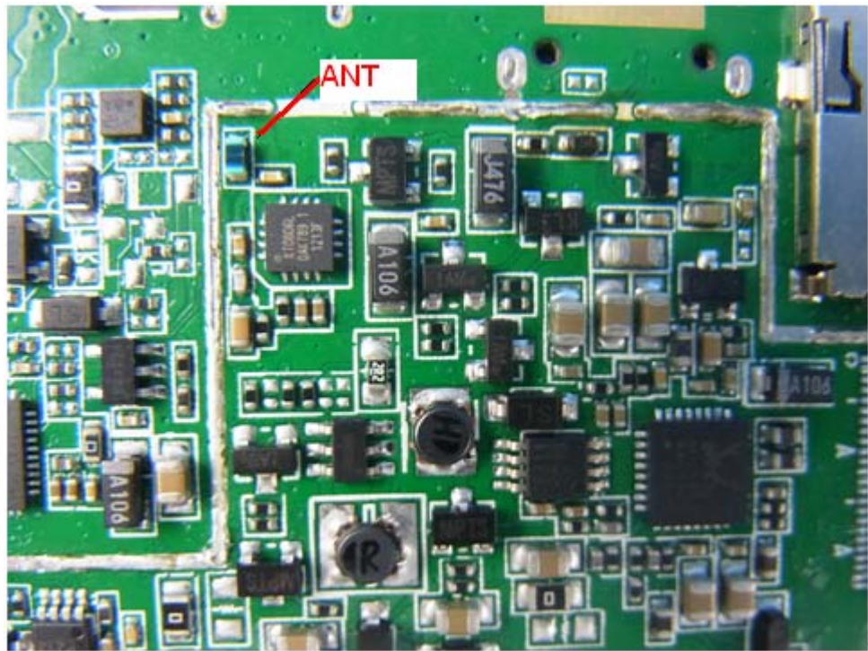
Photo 17 FM ANT
