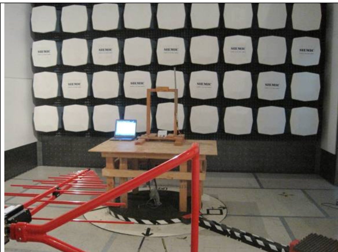
Radiated Emission Test Setup(5dBi Antenna) – Front View
